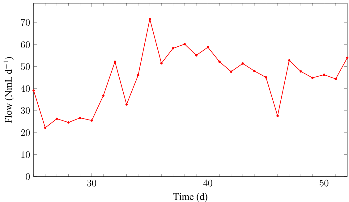
Figure 5.8: Volume flow of \text{CH}_4 \text{NmL d}^{-1} (co-digestion of FW and C-GL)
