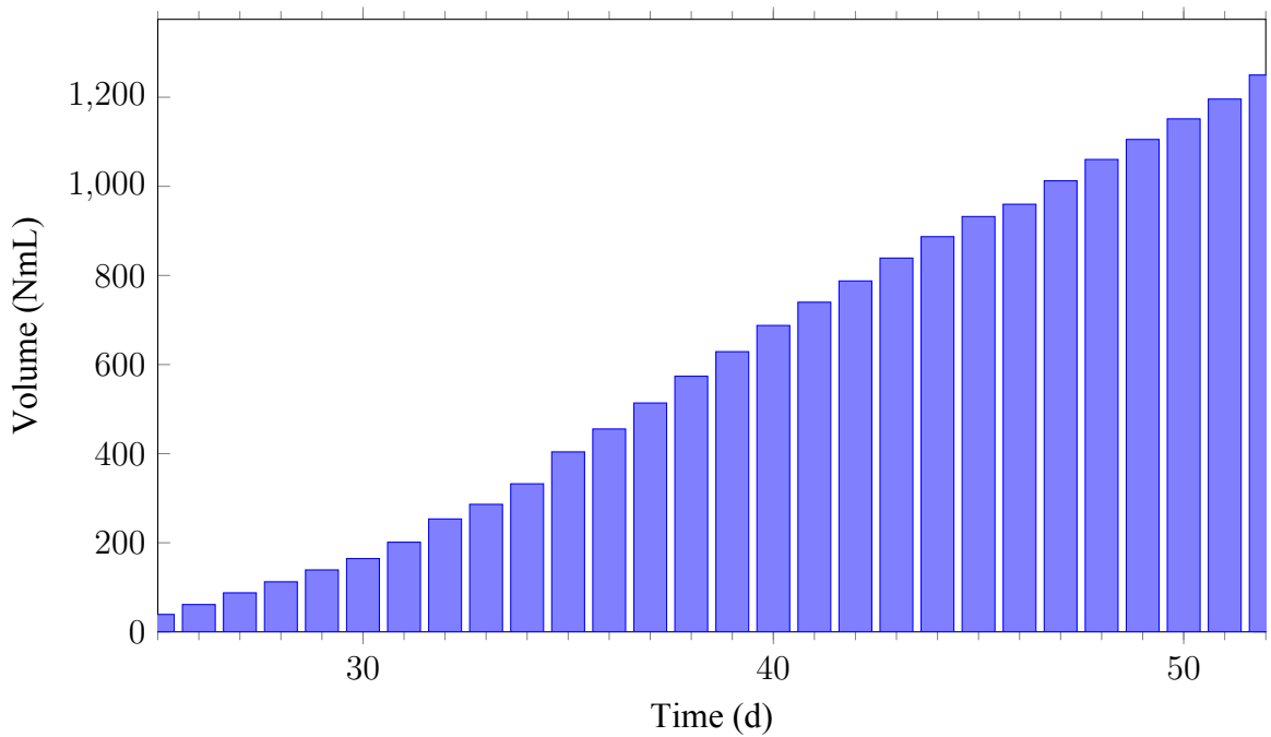
Figure 5.7: Cumulative volume of \text{CH}_4 NmL (co-digestion of FW and C-GL)
