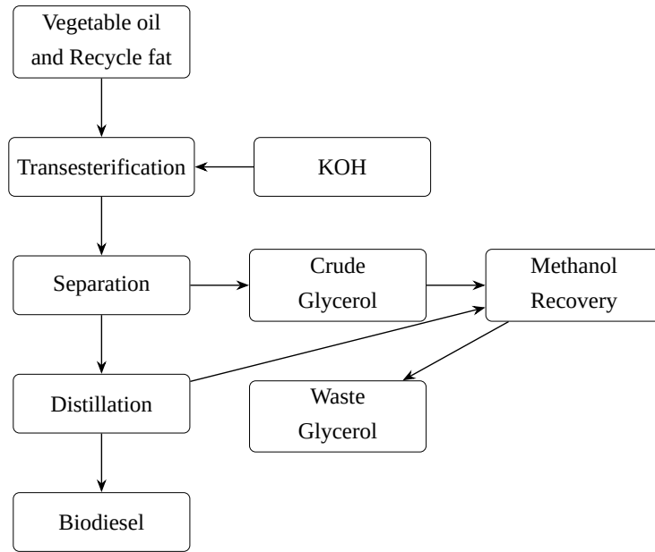
Figure 3.1: Crude glycerol from biodiesel production (Adapted from: Garlapati, Shankar, and Budhiraja (2016))
