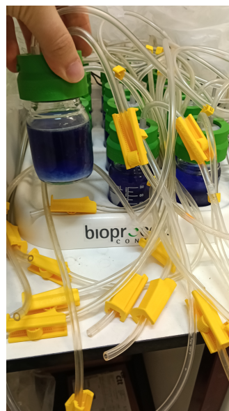
(b) Automatic Methane Potential Test System CO 2 trap
