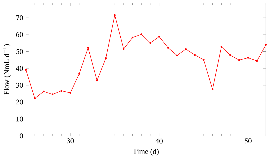
Figure 5.8: Volume flow of CH 4 NmL d -1 (co-digestion of food waste and crude glycerol)
