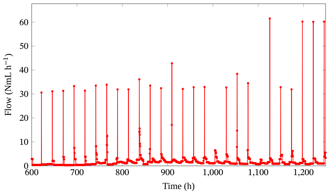
Figure 5.9: Volume flow of CH 4 NmL h -1 (co-digestion of food waste and crude glycerol)
