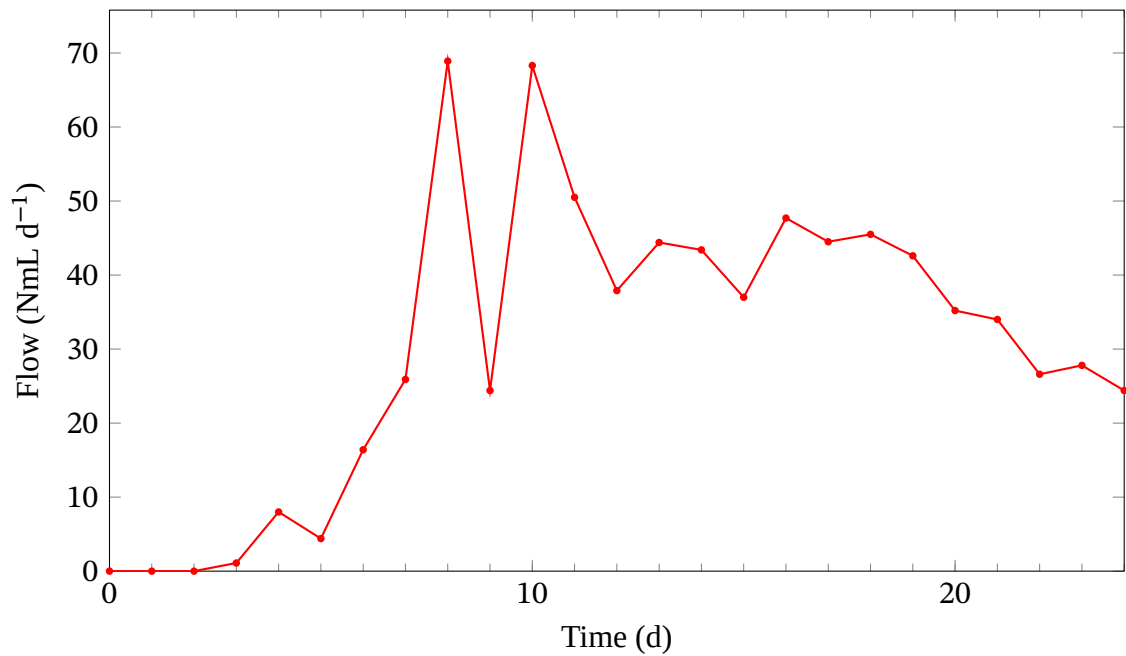
Figure 5.6: Volume flow of \text{CH}_4 \text{NmL d}^{-1} (Adaptation Phase)
