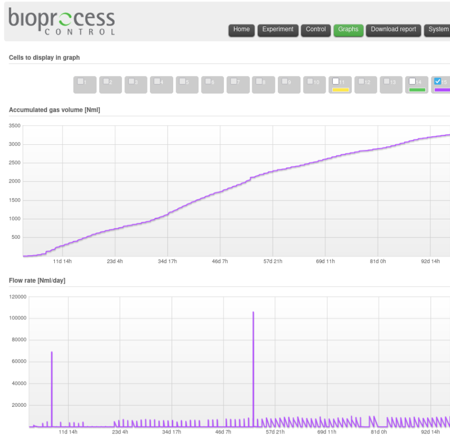
Figure 4.3: Automatic Methane Potential Test System software
