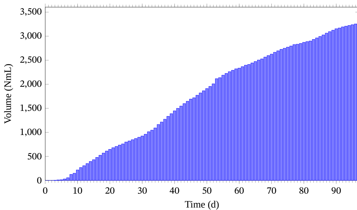
Figure 5.3: Cumulative volume of \text{CH}_4 NmL
