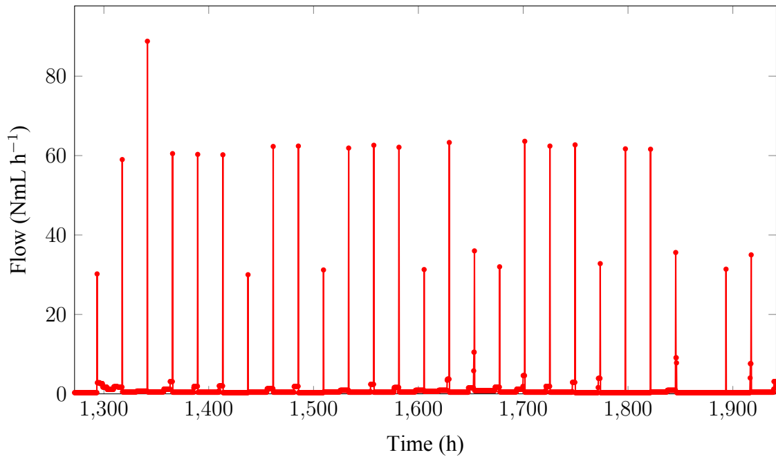
Figure 5.12: Volume flow of \text{CH}_4 \text{NmL h}^{-1} (Anaerobic digestion of C-GL)
