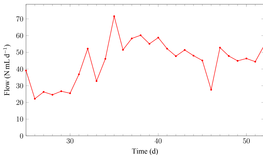
Figure 5.8: Volume flow of \text{CH}_4 N mL d -1 (co-digestion of food waste and crude glycerol)
