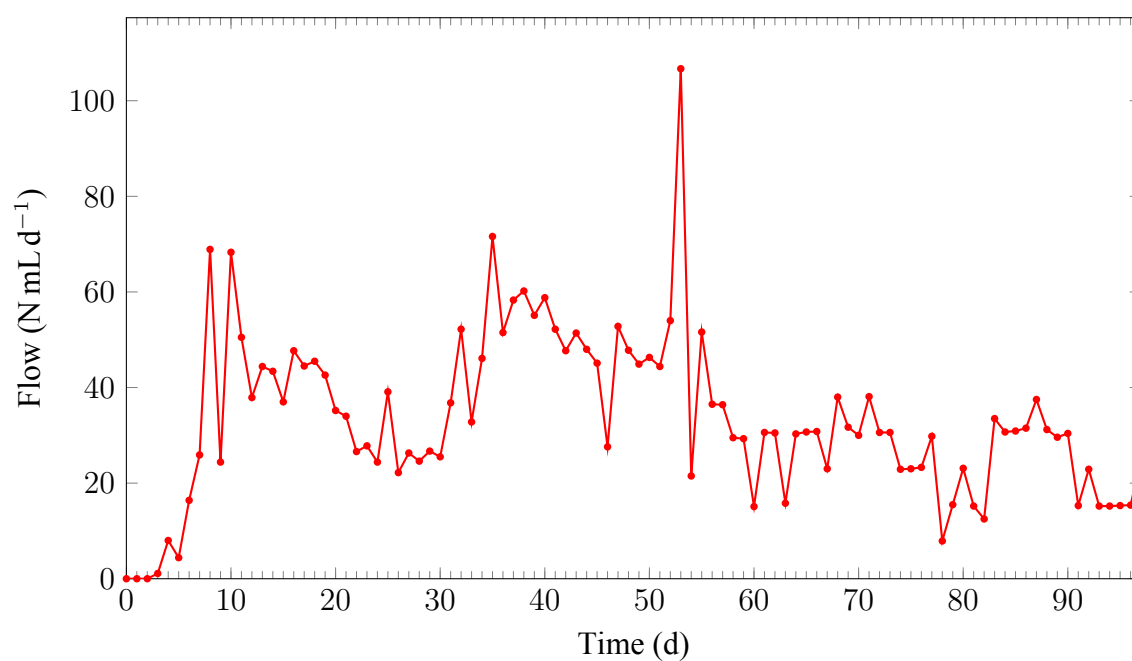
Figure 5.4: Volume flow of \text{CH}_4 \text{N mL d}^{-1}
