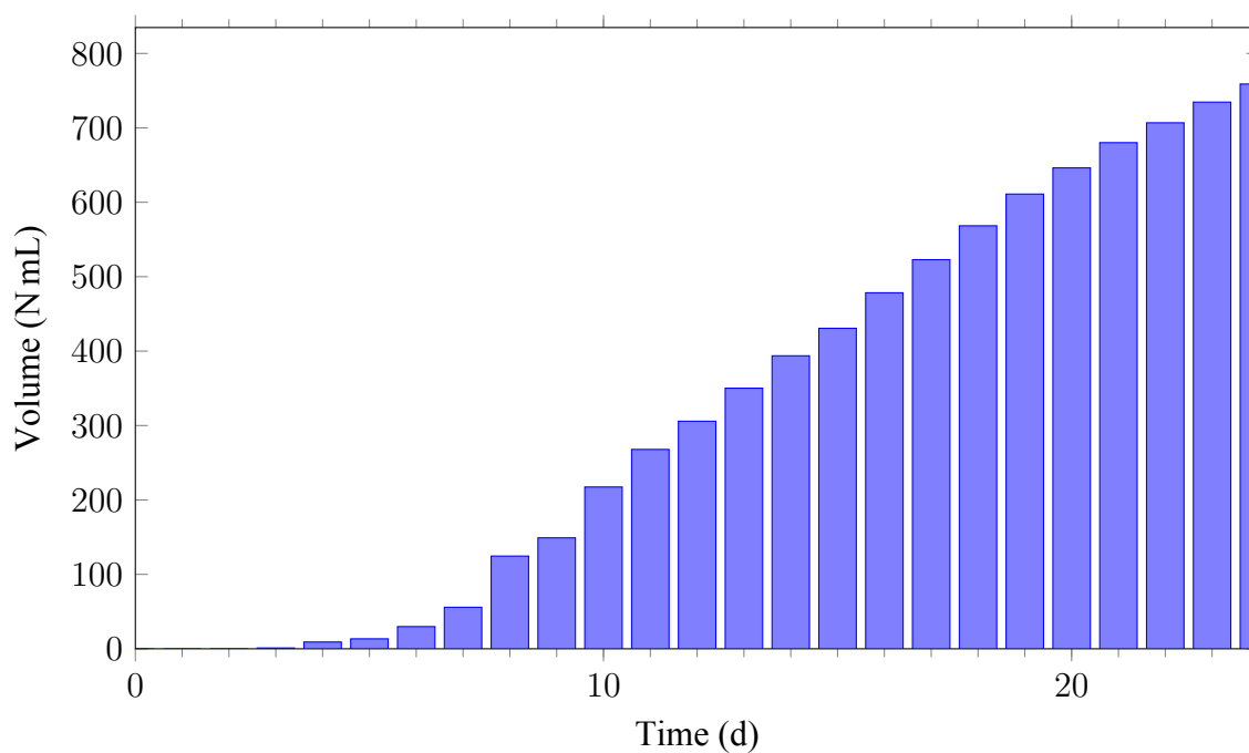
Figure 5.5: Cumulative volume of CH 4 N mL (Adaptation Phase)
