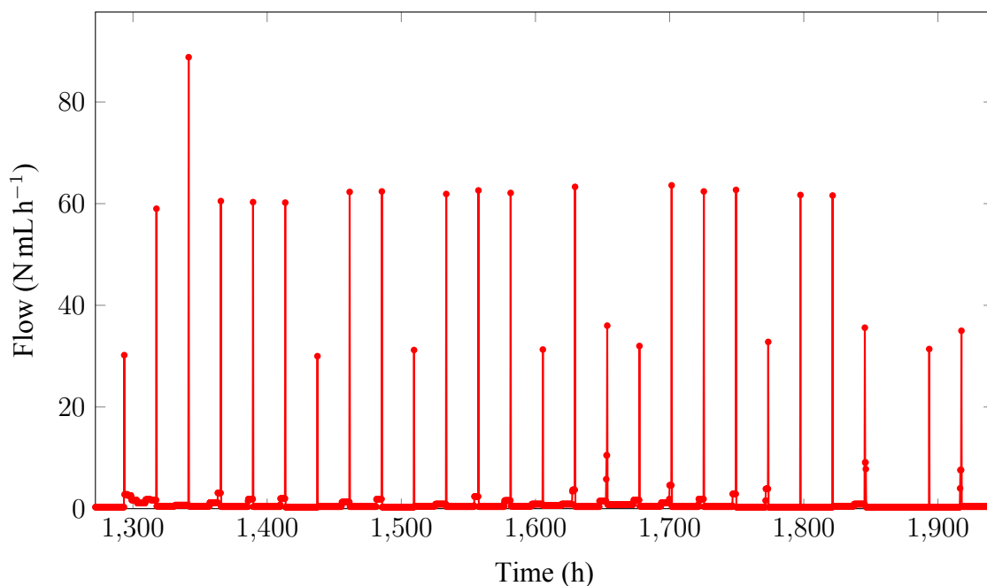
Figure 5.12: Volume flow of CH 4 N mL h -1 (Anaerobic digestion of crude glycerol)
