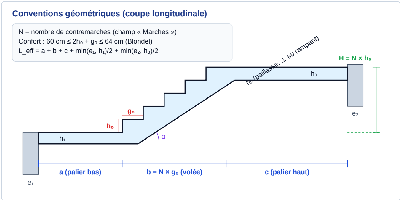
Figure 8 - Conventions de saisie : N contremarches, b = N \times g_0 , H = N \times h_0 .
