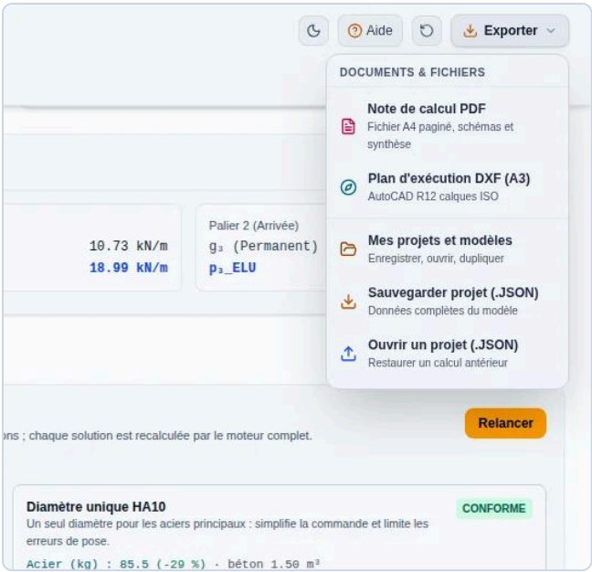
Figure 19 – Menu Exporter.
