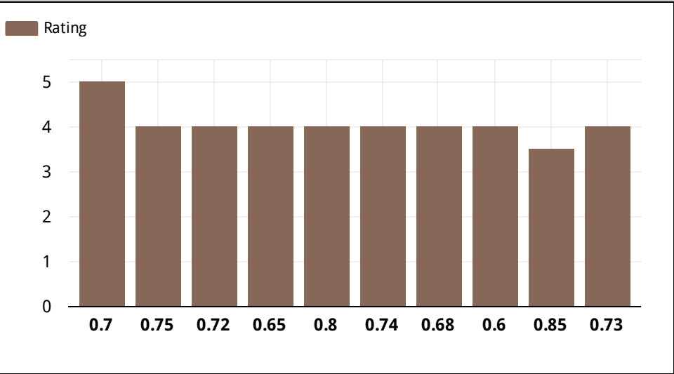
Top 10 Most Used Cocoa Percentages
