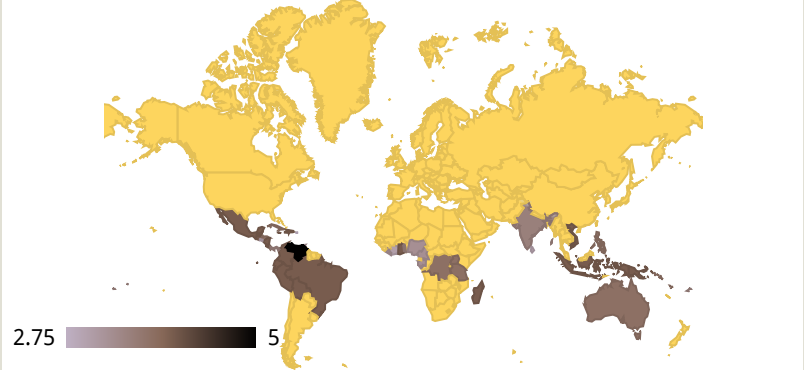
Most Popular Broad Bean Origins (Country)
