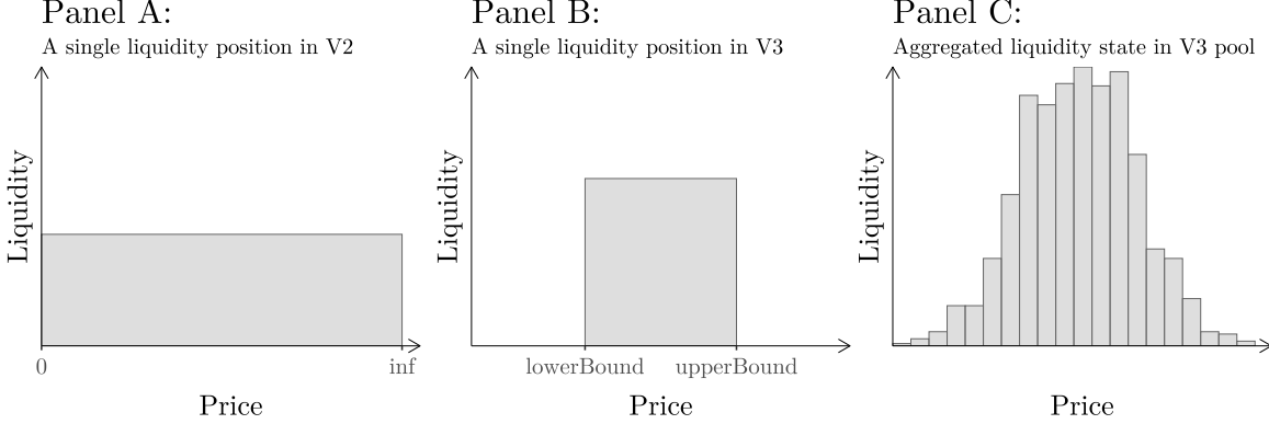
Figure 2: “Liquidity state in Uniswap V2 and V3” adapted from Adams et al. (2021). This figure exemplifies the liquidity states in Uniswap V2 and V3. Panel A shows the liquidity state in a Uniswap V2 pool that provides liquidity across the whole price range. Panel B shows the liquidity distribution of a single, concentrated liquidity position in Uniswap V3 that distributes its liquidity in a price range between a lower bound and an upper bound. Panel C depicts the aggregated liquidity state of multiple liquidity positions in a Uniswap V3 liquidity pool.
