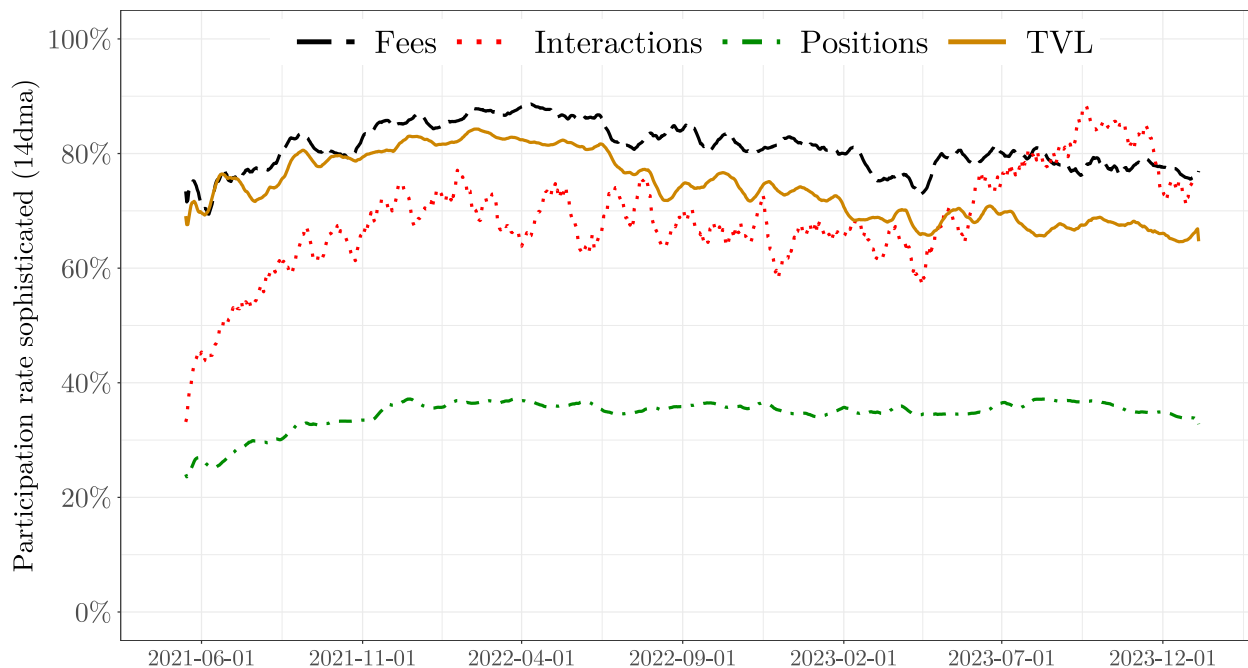
Figure 7: Participation of sophisticated LPs at the protocol level. This figure shows the participation rate of sophisticated market participants across multiple dimensions. Daily pool values are aggregated using a 14 days moving average. Fees is the USD of accrued fees, Interactions is the number of liquidity related transactions, positions is the proportion of fee-collecting liquidity positions and TVL is the total-value locked in USD.
