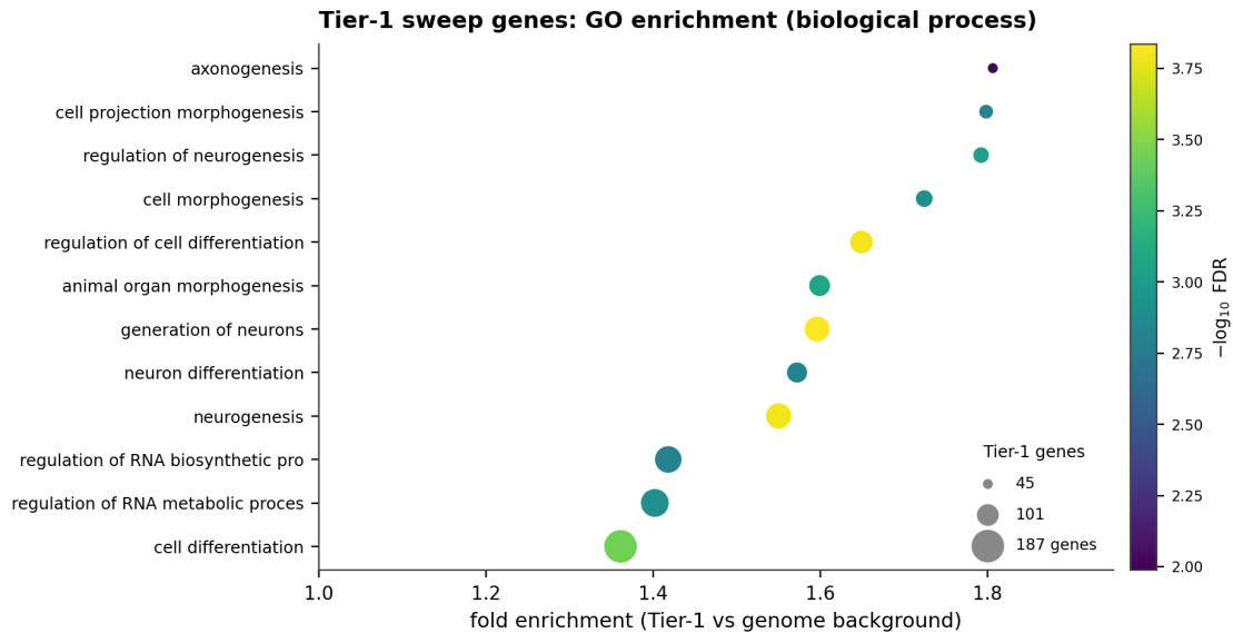
Figure S15: GO enrichment of the Tier-1 sweep genes (biological process) . Each dot is an enriched term: x = fold enrichment, size = number of Tier-1 genes, colour = -\log_{10} \text{FDR} . Two themes dominate — neural development and RNA-regulatory/transcriptional control (table S4).
