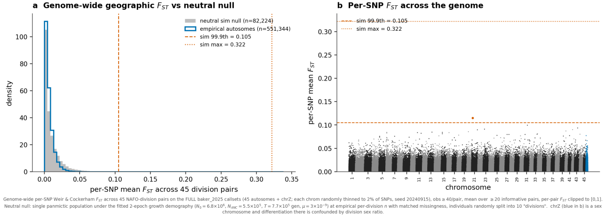
Figure S20: Genome-wide per-SNP F_{ST} finds no differentiation outlier. The window scan of fig. S2 extended to the full per-chromosome callsets (551,344 autosomal SNPs, 2% thinning, covering 12,007 genes). (a) The empirical per-SNP F_{ST} distribution across the 45 division pairs lies entirely within — and slightly narrower than — the coalescent neutral null. (b) Genome-wide, no SNP exceeds the neutral maximum (0.322); a single intergenic SNP on chromosome 21 exceeds the lenient 99.9th percentile (0.105), against \approx 556 expected by chance — i.e. \sim 555\times fewer outliers than the false-positive rate. Zero genic outliers, hence no functional enrichment. Extreme panmixia is confirmed at genome scale, and no local-adaptation signal is present that the diversity-based sweep scans could have missed. (chrZ, blue in (b), is confounded by division sex ratios and shown for completeness.)
