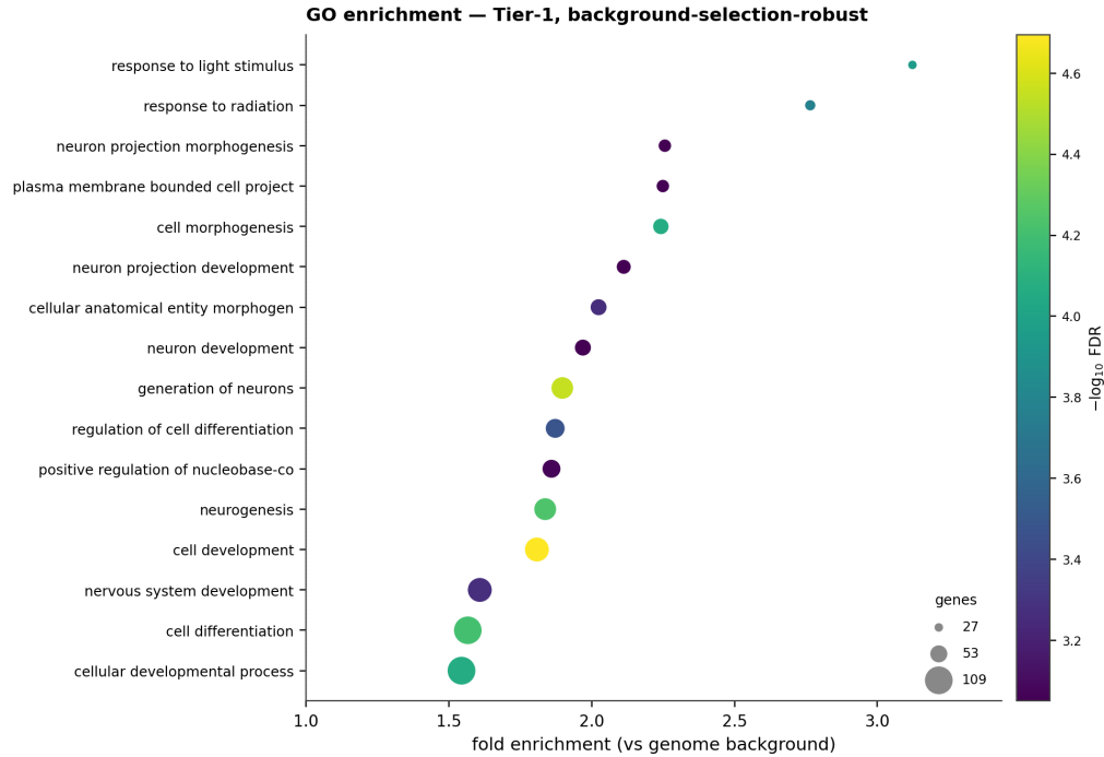
Figure S19: GO enrichment of the background-selection-robust Tier-1 sweep genes (GSEA-style dot plot; top terms by FDR). Each dot is an enriched biological-process term: x = fold enrichment, size = number of genes, colour = -\log_{10} FDR. After BGS screening the neural-developmental and RNA-regulatory enrichment strengthens and a photoreception signal (response to light/radiation) appears; the full and hard-sweep Tier-1 dot plots ( supp_gsea_tier1.png , supp_gsea_hard.png ) are provided with the source.
