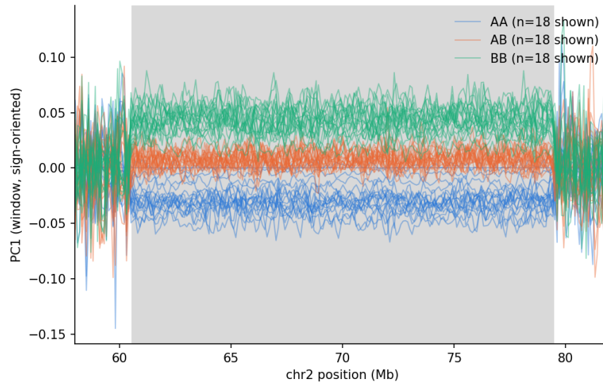
Figure S3: Windowed PCA across chromosome 2 localising the differentiated block.
