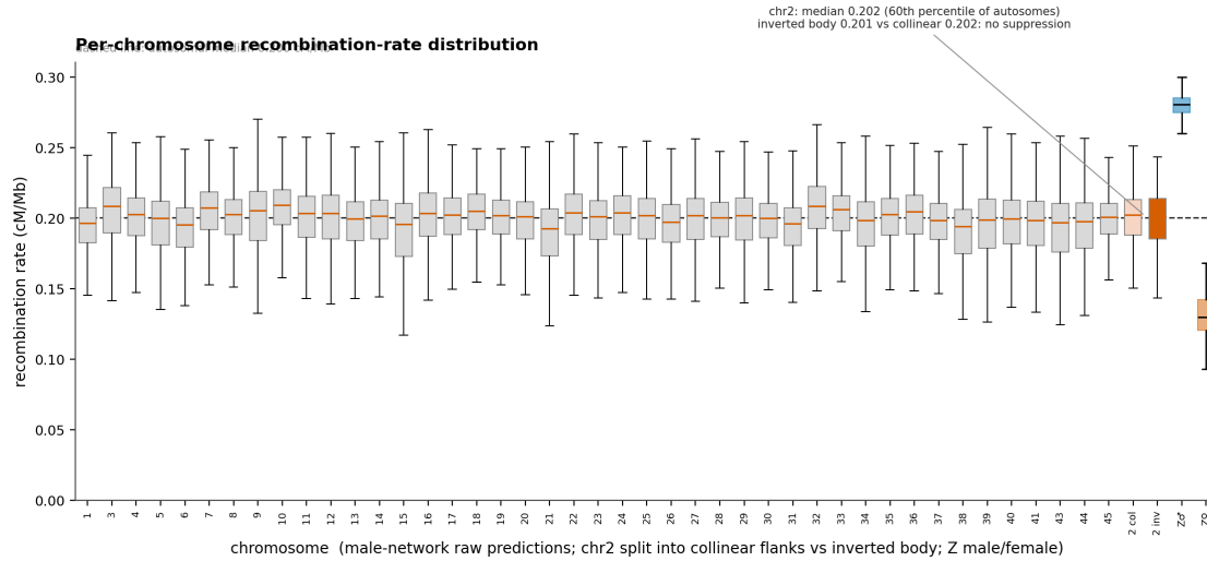
Figure S12: Per-chromosome recombination-rate distribution (ReLERNN). All boxes are raw predictions of the male autosomal network so that chromosomes are compared on the same footing: the 43 scanned autosomes, chromosome 2 split into its collinear flanks and the inverted body (60.54–79.50 Mb), and the Z (male and female runs). Chromosome 2 is an ordinary autosome (median 0.202 vs 0.200 cM/Mb genome-wide, the 60th percentile of per-chromosome medians) and the inverted body is not depressed relative to the flanks (0.2015 vs 0.2023): the estimator reads within-window linkage disequilibrium at the \sim 19 -kb scale and does not register the arrangement-level barrier, which is shown directly by main-text Fig. 3b and Supplementary Figs. S4 and S5. The female autosomal map collapses to a near-constant (Supplementary Fig. S22b) and is not shown here.
