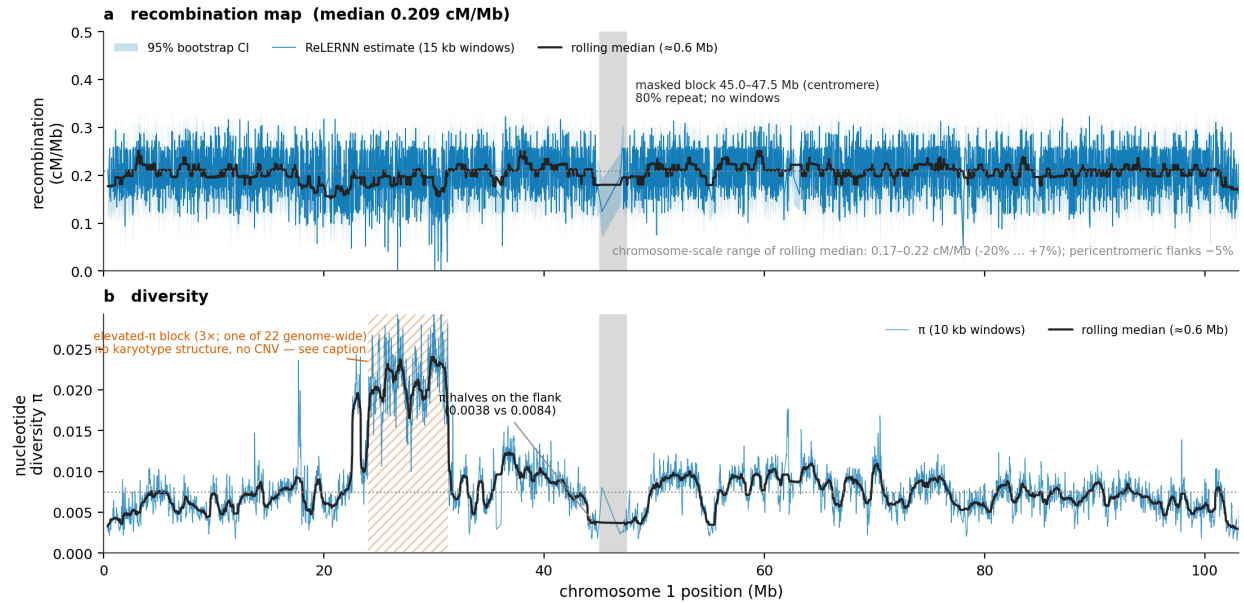
Figure S22: The chromosome-1 recombination landscape, and what the LD-based map does not resolve. (a) ReLERNN estimate in 15 kb windows with 95% bootstrap CIs and a 0.6-Mb rolling median (median 0.209 cM/Mb). The shaded 2.5-Mb block at 45.0–47.5 Mb is 80% repeat sequence (vs 52% chromosome-wide), is almost entirely masked, and carries no ReLERNN windows: the centromere. In the accessible pericentromeric flanks the estimate dips only \sim 5\% , and across the whole 103 Mb the rolling median spans just 0.17–0.23 cM/Mb ( -20\% to +7\% of the median) — the map’s chromosome-scale dynamic range is compressed, so centromeric suppression cannot be resolved and the “nearly uniform” landscape is in part an estimator ceiling. (b) Nucleotide diversity \pi in 10 kb windows halves on the flank of the masked block — the pericentromeric signature that the recombination estimate in (a) does not show. The block of tripled \pi at 24–31 Mb (hatched) is one of 22 such \geq 1 -Mb blocks genome-wide. It is not a structural polymorphism: a local PCA shows no karyotype clusters (its Gaussian-mixture “clusters” track coverage, and heterozygosity is flat across them, unlike the chr2 inversion), there is no excess heterozygosity, no loss to the excess-heterozygosity filter, and the per-individual read-depth ratio to flanking sequence is tight and unimodal (median 0.95, IQR 0.94–0.97; no duplication carriers); its folded allele-frequency spectrum is identical to the flanks. It is gene-poor (coding fraction 0.001), only 35% alignable to I. coindetii (vs 87–89% in flanks) and 1.65-fold more divergent where alignable (3.3% vs 1.9–2.1%), and low-coverage I. argentinus reads call \sim 3\times more variants in it — a fast-evolving, largely lineage-specific gene desert (elevated mutation input plus relaxed linked selection), not an inversion or introgression.
