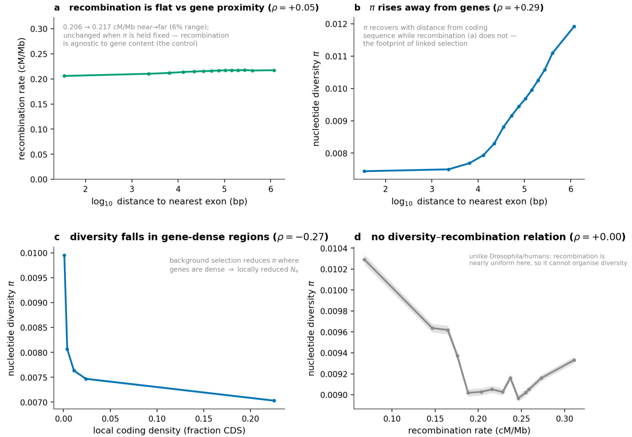
Figure S17: Recombination, gene proximity and the efficacy of selection. Per-window statistics ( \sim 50 kb windows, autosomes). (a) The control: recombination rate is essentially flat across distance from the nearest exon (0.206 \rightarrow 0.217 cM/Mb near \rightarrow far, a \sim 6\% range; Spearman \rho = +0.05 , unchanged when \pi is held fixed, partial \rho = +0.06 ) — recombination is agnostic to gene content, as it should be. (b) Nucleotide diversity \pi , by contrast, rises steeply with distance from coding sequence ( \rho = +0.29 ; +43\% near \rightarrow far): the footprint of linked selection. (c) \pi falls with local coding density ( \rho = -0.27 ) — background selection reduces diversity where genes are dense, i.e. a locally reduced effective size, and it is gene-density-driven . (d) There is no diversity–recombination relationship ( \rho \approx 0 ), unlike Drosophila and humans, because recombination is nearly uniform genome-wide (0.2–0.24 cM/Mb) and cannot organise diversity here. Linked selection in Illex illecebrosus is thus structured by gene density and gene proximity rather than by the recombination-rate axis.
