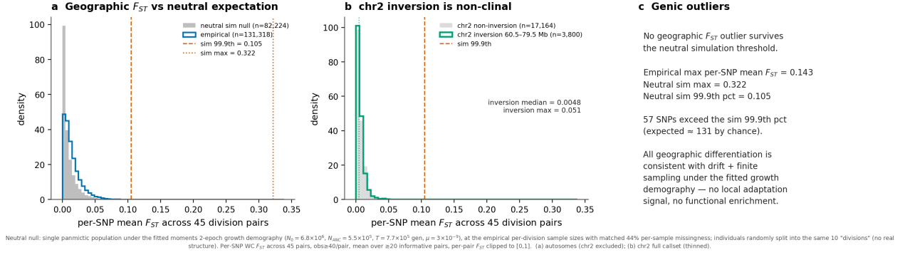
Figure S2: No geographic differentiation beyond genetic drift and no local adaptation signal. Per-SNP Weir–Cockerham F_{ST} across all 45 NAFO-division pairs (well-genotyped sites, \geq 40 observed haplotypes per pair, per-SNP mean over \geq 20 informative pairs). (a) The empirical distribution (blue) lies entirely within a coalescent neutral null (grey), which is a single panmictic population simulated under the fitted growth demography ( N_0 = 6.8 \times 10^6 , N_{ANC} = 5.5 \times 10^5 , \mu = 3 \times 10^{-9} ) at the empirical per-division sample sizes with the matched 44% missingness, split at random into ten “divisions”. Empirical max F_{ST} = 0.143 vs neutral max 0.322. Only 57 SNPs exceed the neutral 99.9th percentile (0.105) against \approx 131 expected by chance, fewer than the false-positive rate. Drift, finite sampling and missingness fully explain the observed differentiation. (b) On chromosome 2, the inverted region (green) is geographically indistinguishable from the collinear remainder (median F_{ST} \approx 0.005 ), so the inversion is non-clinal and its F_{ST} \approx 0.37 is between karyotypes, not geography. (c) No SNP survives the neutral threshold, so a scan for local adaptation that the diversity-based sweep tests could miss returns no candidates. (The autosomal panel samples a fixed 400 kb window per chromosome. The distribution and threshold conclusion is robust, but a genome-wide genic-outlier scan would require per-chromosome F_{ST} on the full callsets.)
