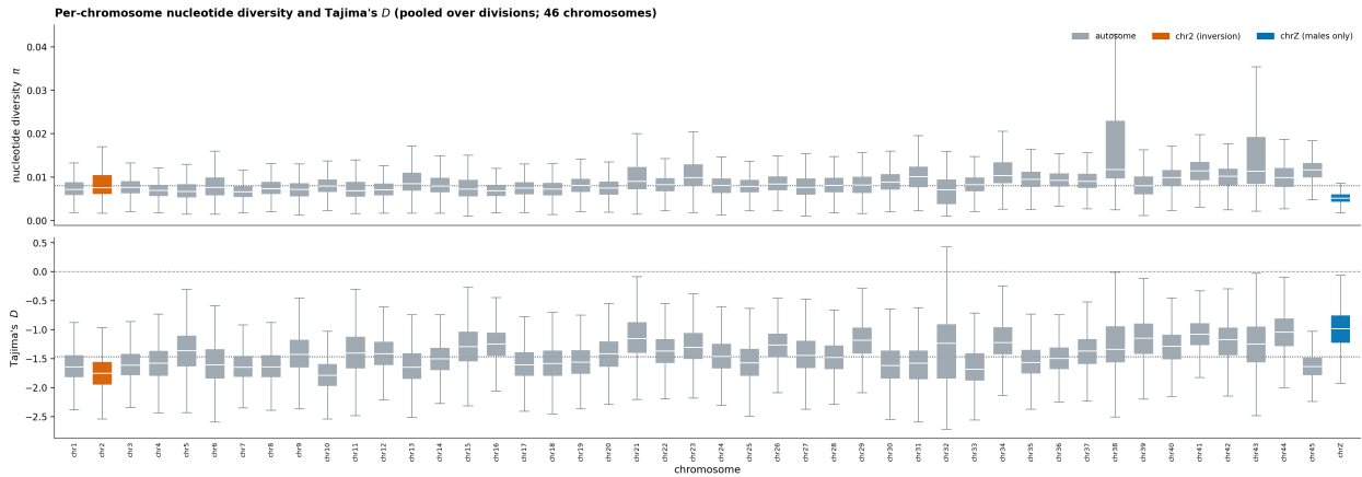
Figure S9: Per-chromosome diversity. Distribution of nucleotide diversity \pi (top) and Tajima's D (bottom) across 50 kb windows, one box per chromosome (pooled over the ten NAFO divisions, for all 46 chromosomes, the 45 autosomes plus chrZ). Diversity is uniform and D is strongly negative genome-wide, the signature of expansion. Two chromosomes stand apart. Chromosome 2 (the inversion, orange) carries an inflated upper tail of \pi and more-negative D from the segregating arrangements, and chrZ (blue, computed in the 330 hemizygous-informative males only, as females are Z-haploid) has reduced diversity ( \pi median 0.005 vs \sim 0.008 autosomal, \approx 0.63\times ) as expected for a sex chromosome.
