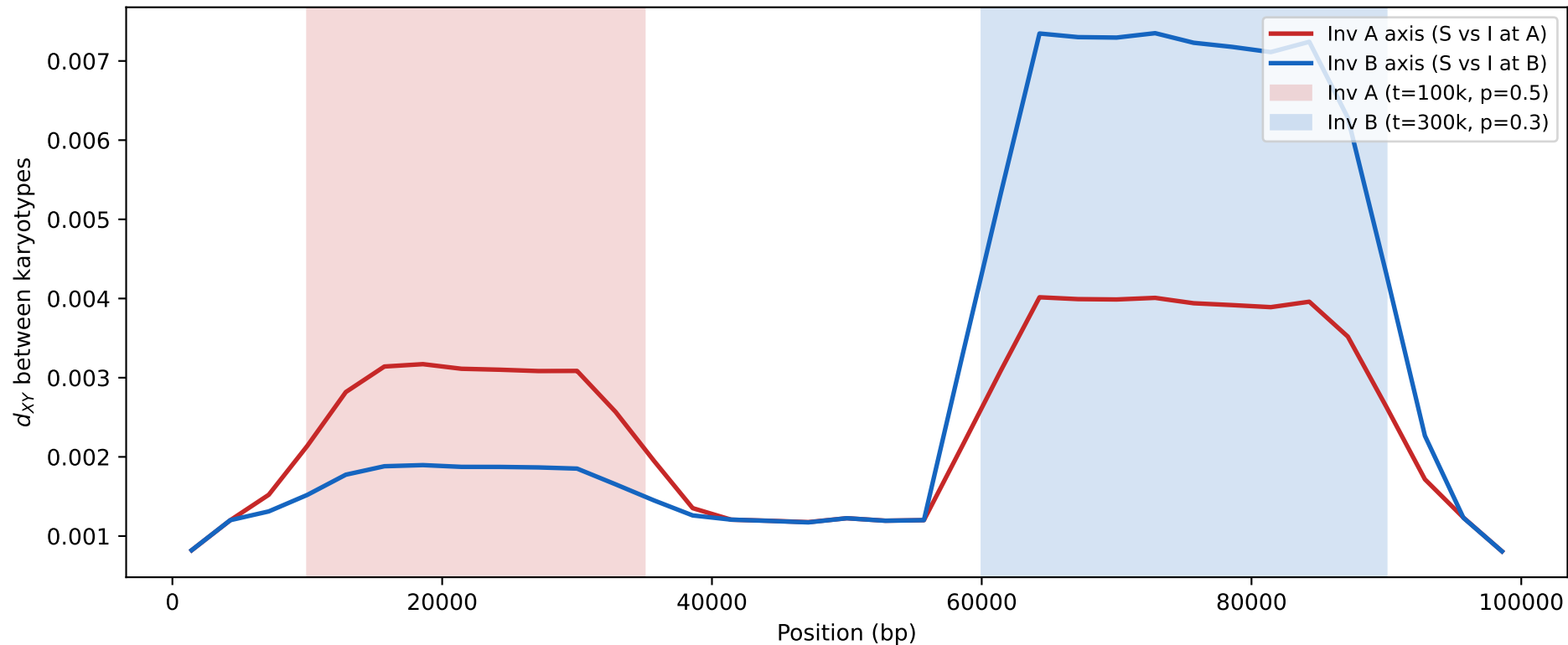
Two independent inversions — each gives its own cross-karyotype barrier signal
