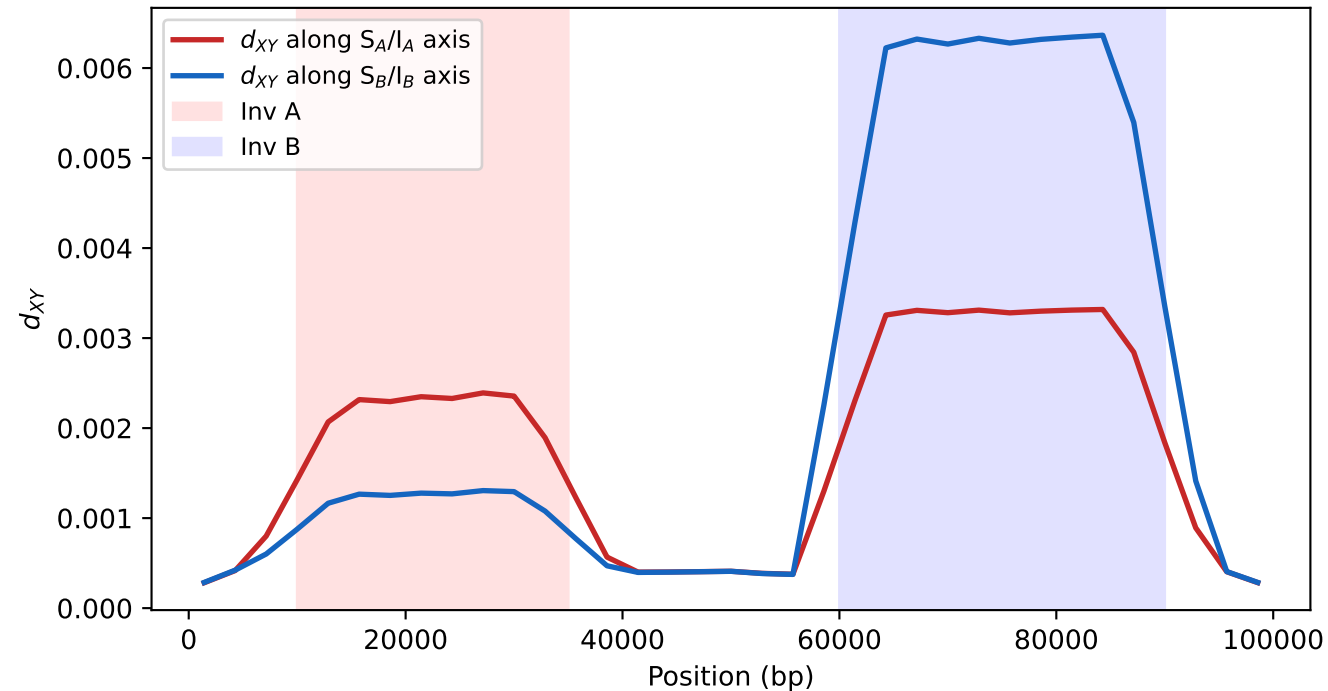
A. Between-karyotype divergence
