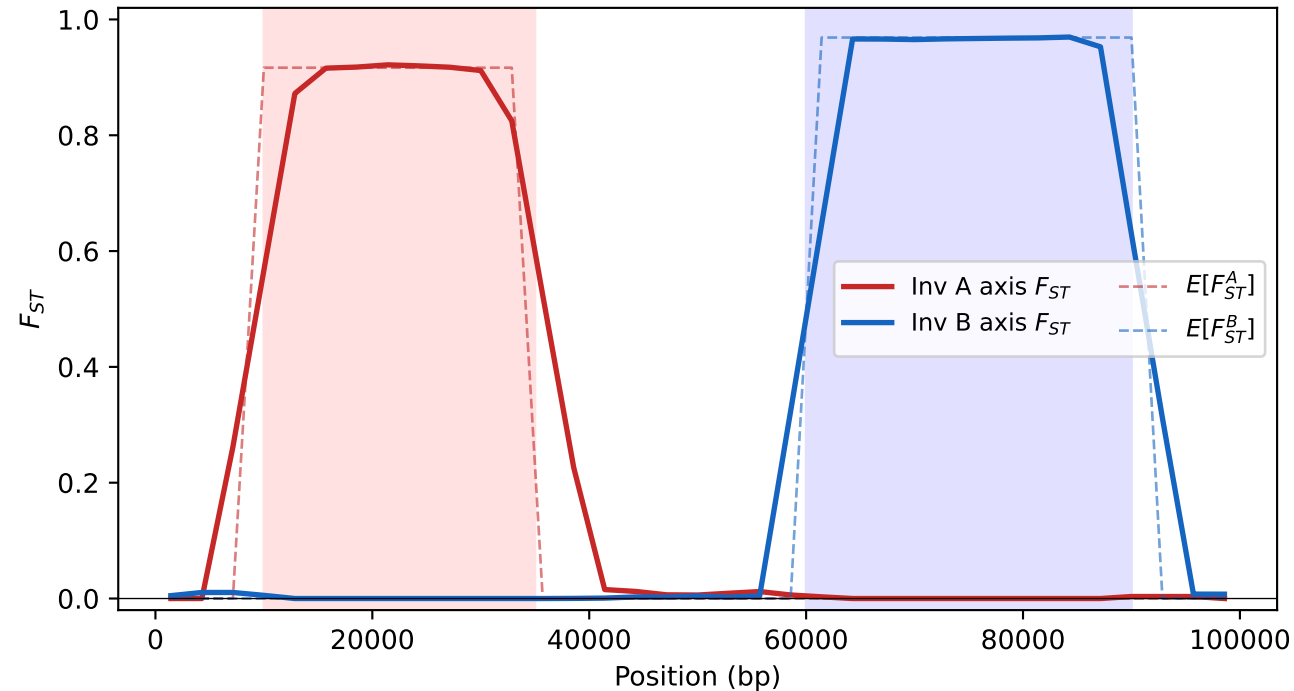
B. Two-axis Hudson F_{ST}
