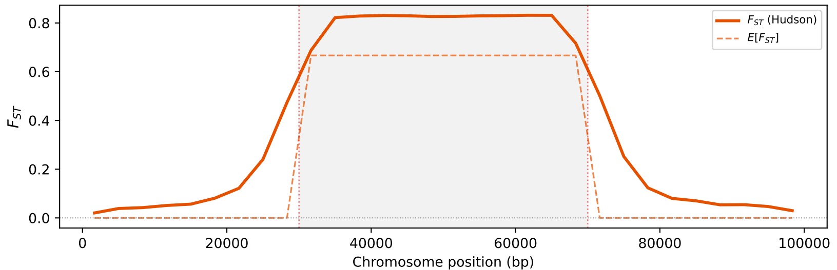
C. Hudson F_{ST} (relative differentiation)
