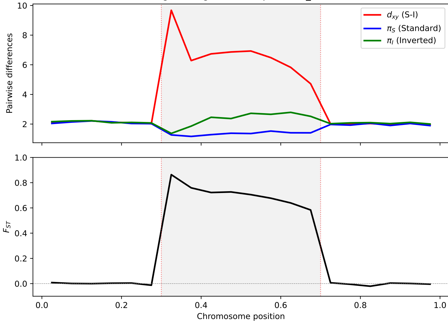
Inversion divergence signal ( n=10 , \rho=100 , t_{\text{inv}}=20 , c=0.01 )
