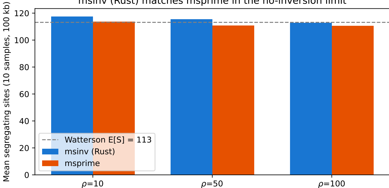
Figure 2. msinv validation against msprime in the no-inversion limit. Mean number of segregating sites from 10 haploid samples across 100 replicates at three recombination rates ( \rho = 4N_e rL ). Without an inversion, msinv produces the same distribution of genealogies as msprime — the two are statistically indistinguishable. Dashed line: Watterson expectation E[S] = \theta \sum_{i=1}^{n-1} 1/i = 113 . Parameters: N_e=10,000 , L=100 kb, \mu=1e-8 , n=10 , 100 replicates per \rho . Command: pixi run -e all python examples/make_figures.py
