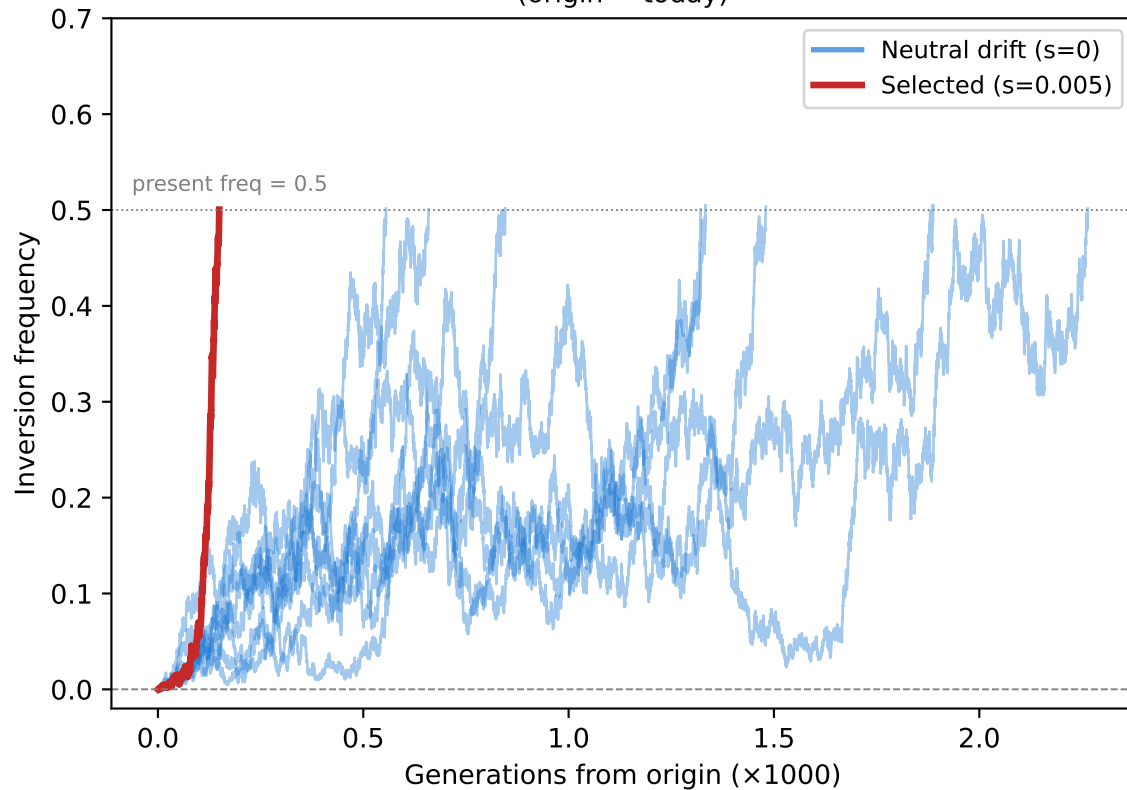
Figure 5. Forward-in-time Wright-Fisher trajectories for inversion frequency. (A) Example trajectories from 1/(2N) to a present frequency of 0.5. Neutral drift (blue, 8 runs) takes highly variable paths; positive selection ( s=0.005 , red) reaches the same frequency much faster. (B) Distribution of inversion ages (time from origin to reaching p=0.5 ) across 50 neutral trajectories. Even for the same present frequency, inversion ages vary by orders of magnitude — this motivates ABC inference rather than point estimates of t_{\text{inv}} . Parameters: N_e=10,000 , 10 gen/yr, p_{\text{target}}=0.5 . Command: pixi run -e all python examples/make_figures.py
