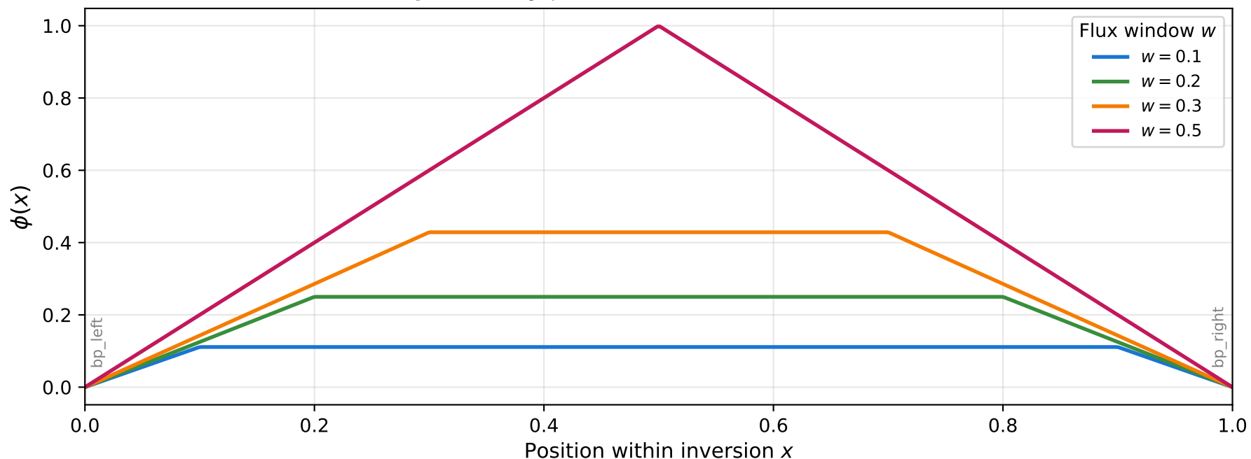
A. Theoretical flux-transfer probability \phi(x) = \min(x, 1 - x, w)/(1 - w)
