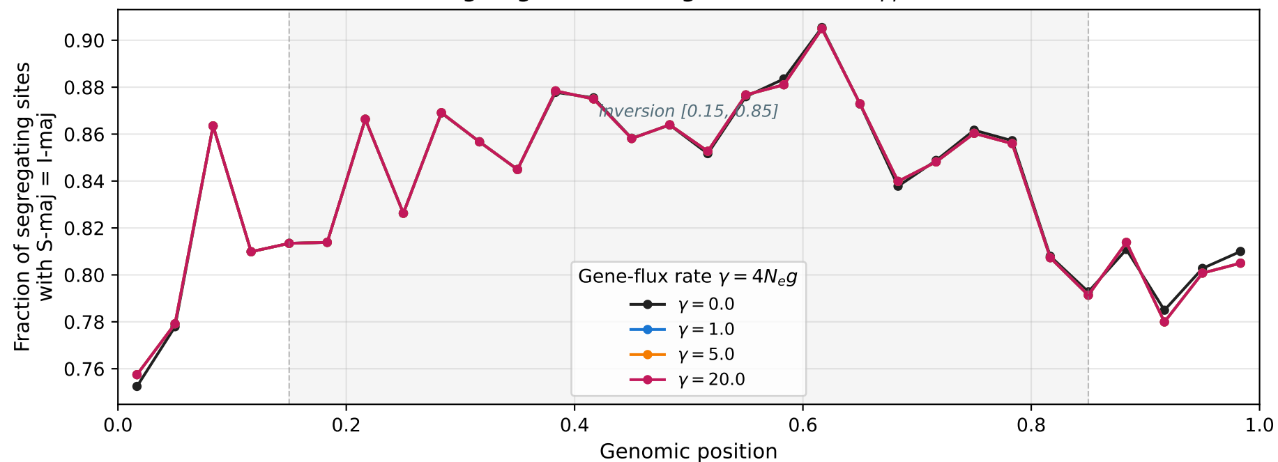
B. Simulated S-I allele-sharing vs gamma (mixing increases with \gamma\phi(x)t )
