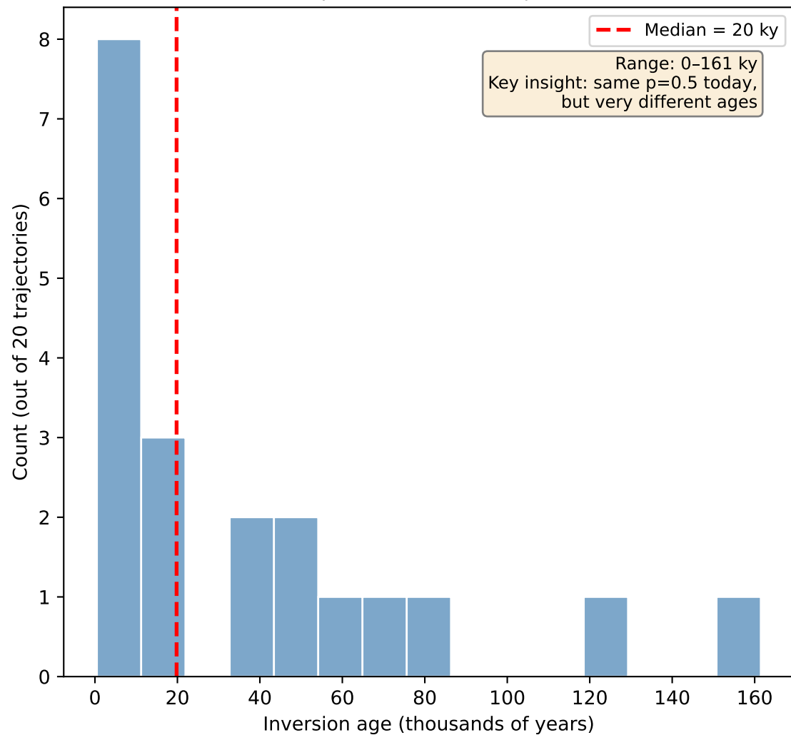
B. Inversion age depends on stochastic history (20 independent neutral trajectories)
