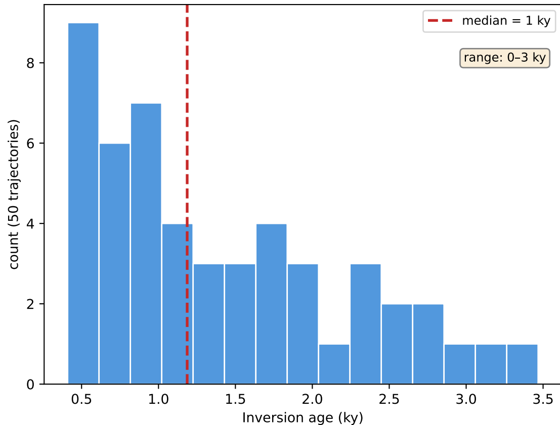
B. Inversion age varies widely (same present freq, different histories)
