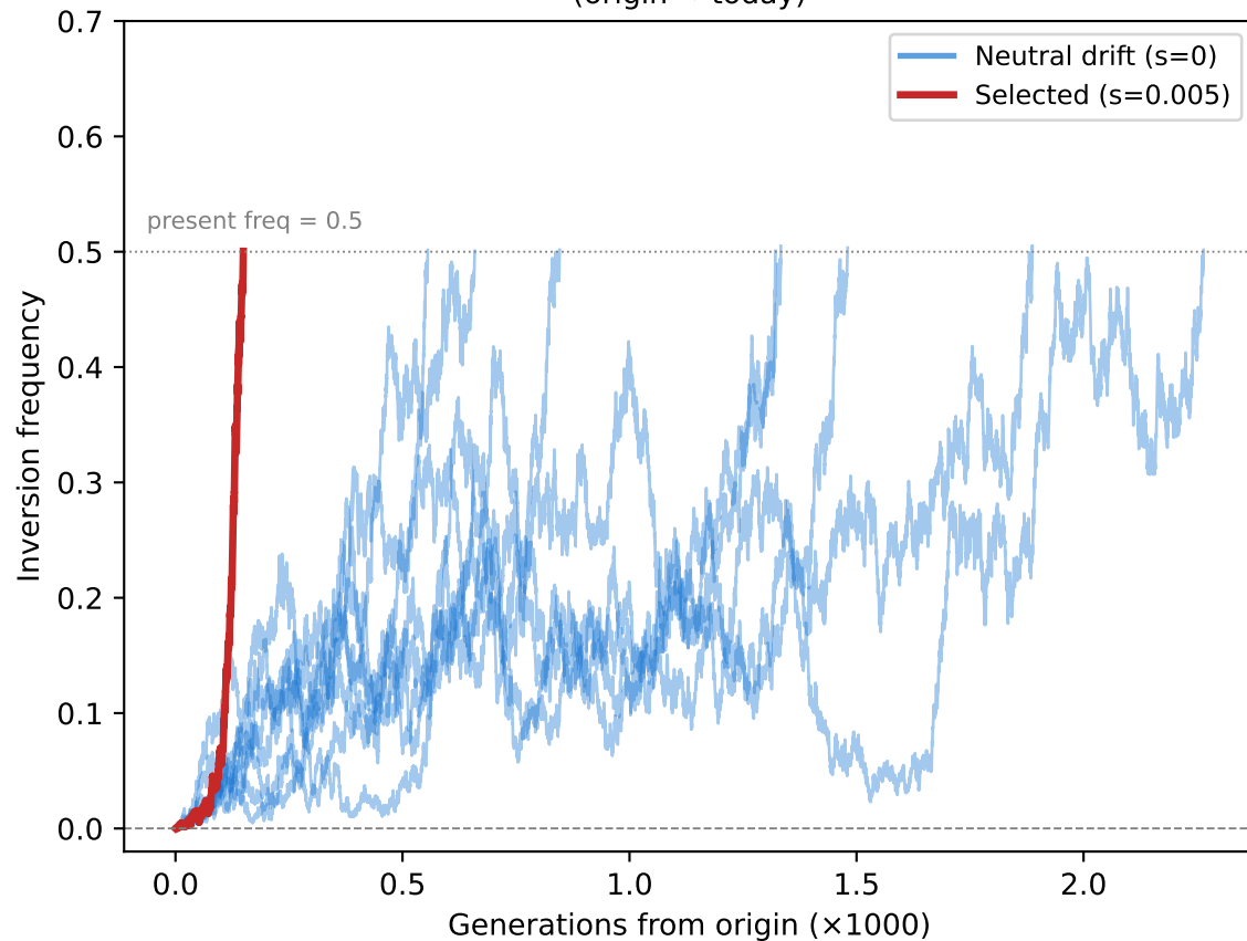
A. Forward-in-time WF trajectories (origin \rightarrow today)
