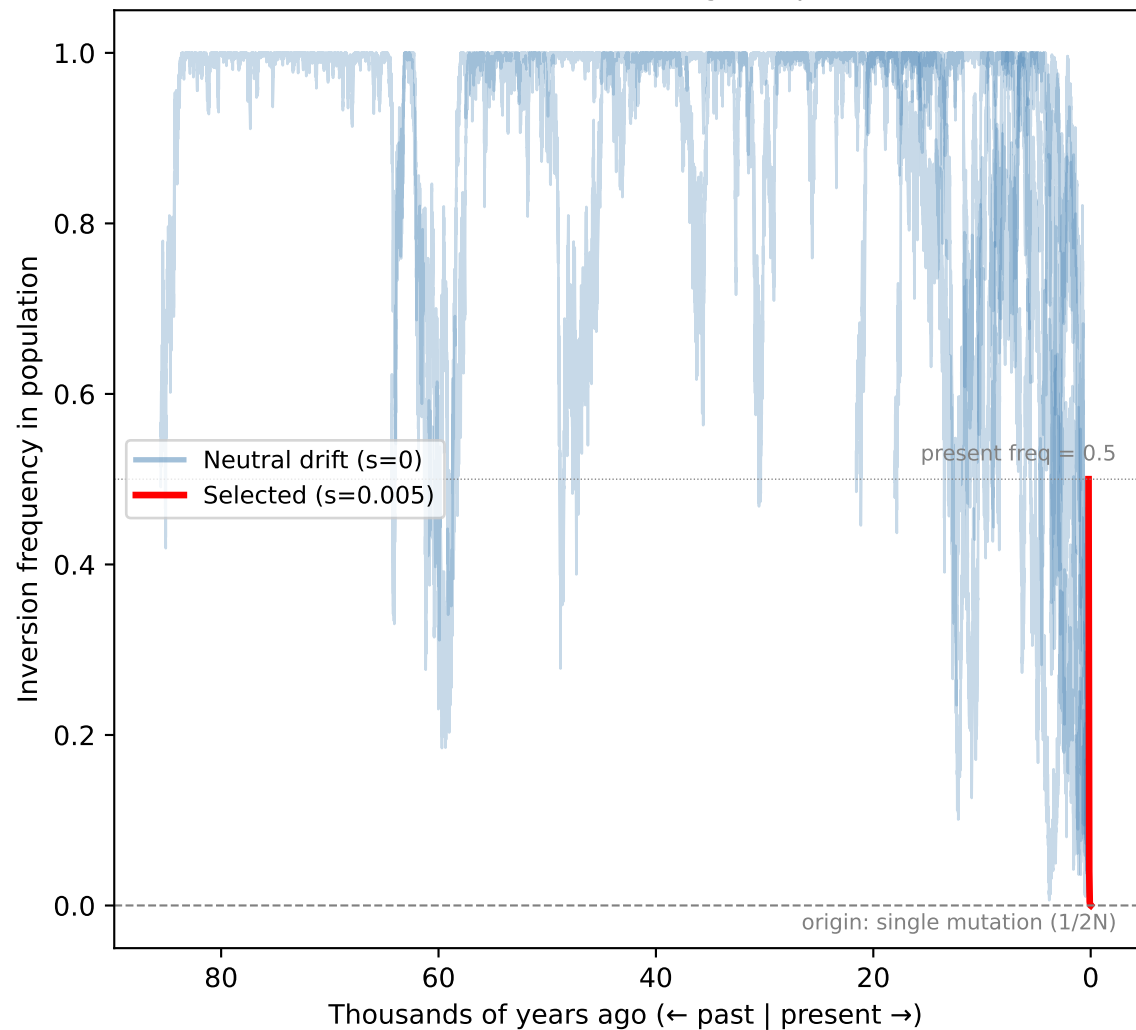
A. How inversions establish (forward in time, from origin to present)
