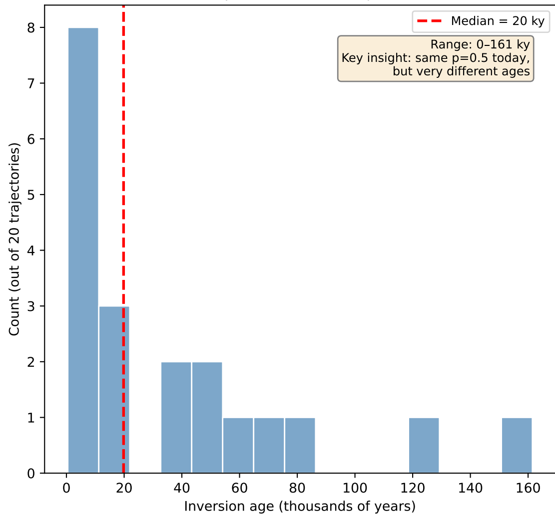
B. Inversion age depends on stochastic history (20 independent neutral trajectories)
