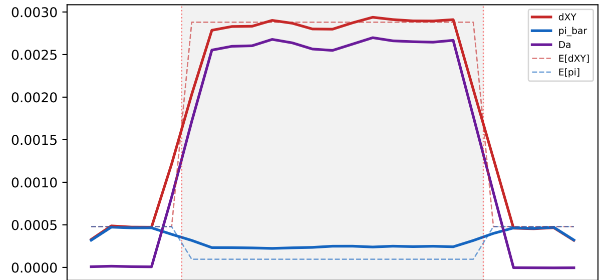
Human MAPT H1/H2-like (Ne=10k)
