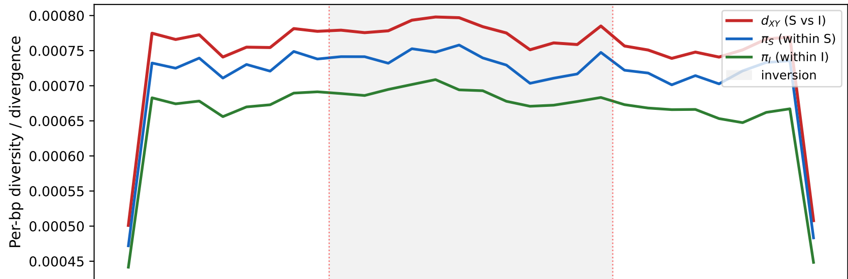
A. Inversion divergence signal (Ne=50,000, t_inv=200k gen, n_S=8, n_I=8, 100 reps)
