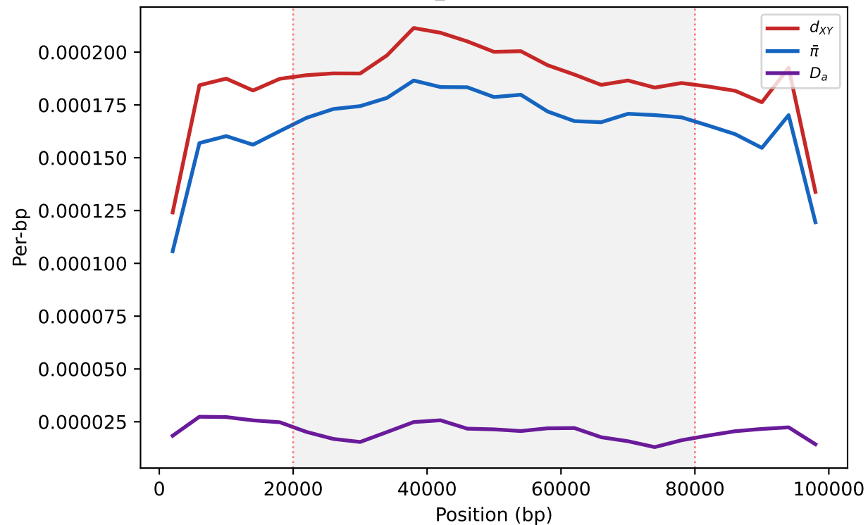
Human MAPT H1/H2-like (Ne=10k, t_inv=3 Myr / 100k gen)
