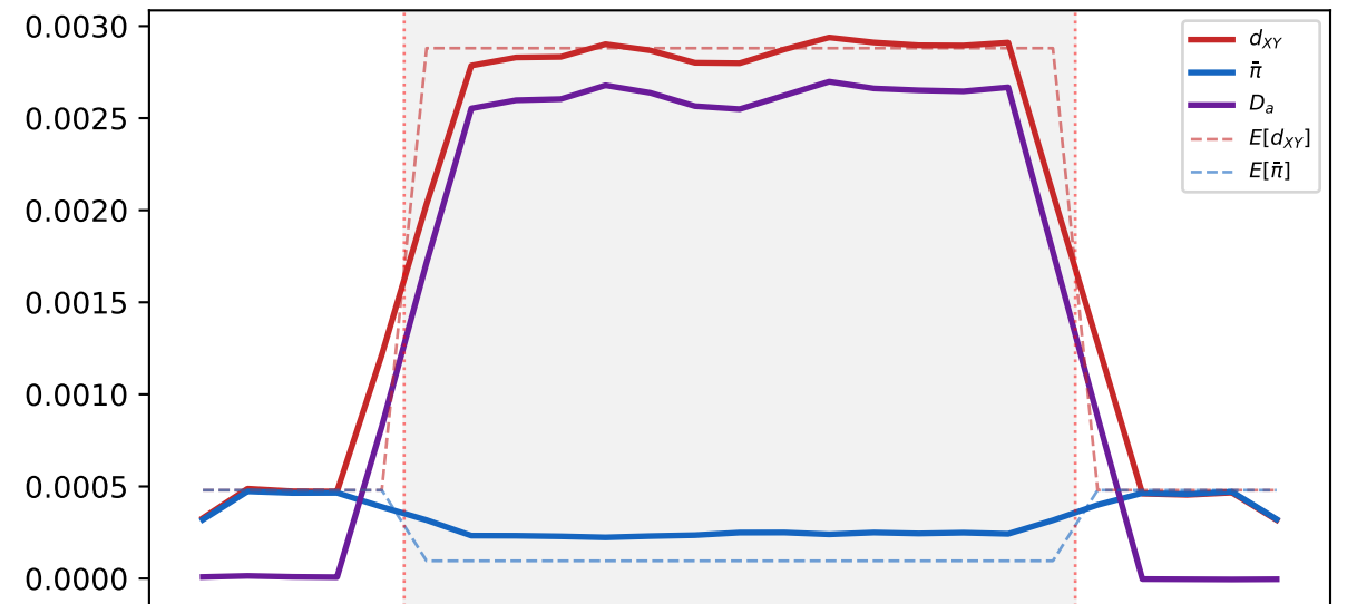
Human MAPT H1/H2-like (Ne=10k, t_inv=100k gen)
