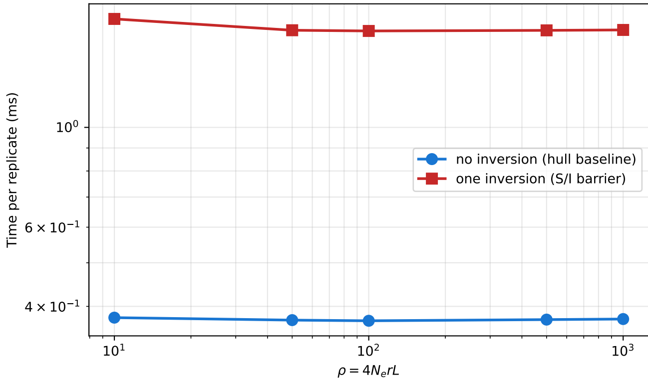
Hull simulator scaling (n=10, L=100kb)
