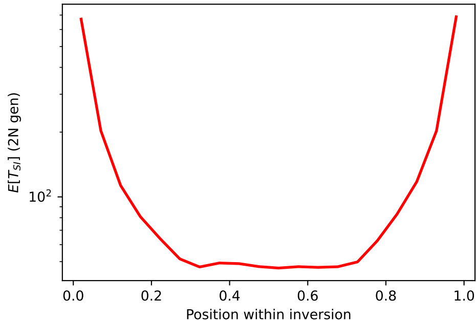
Coalescence time between arrangements ( \rho=10 , c=0.01 )
