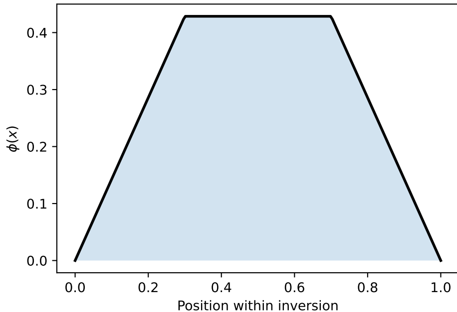
Gene flux probability (flux window w=0.3 )
