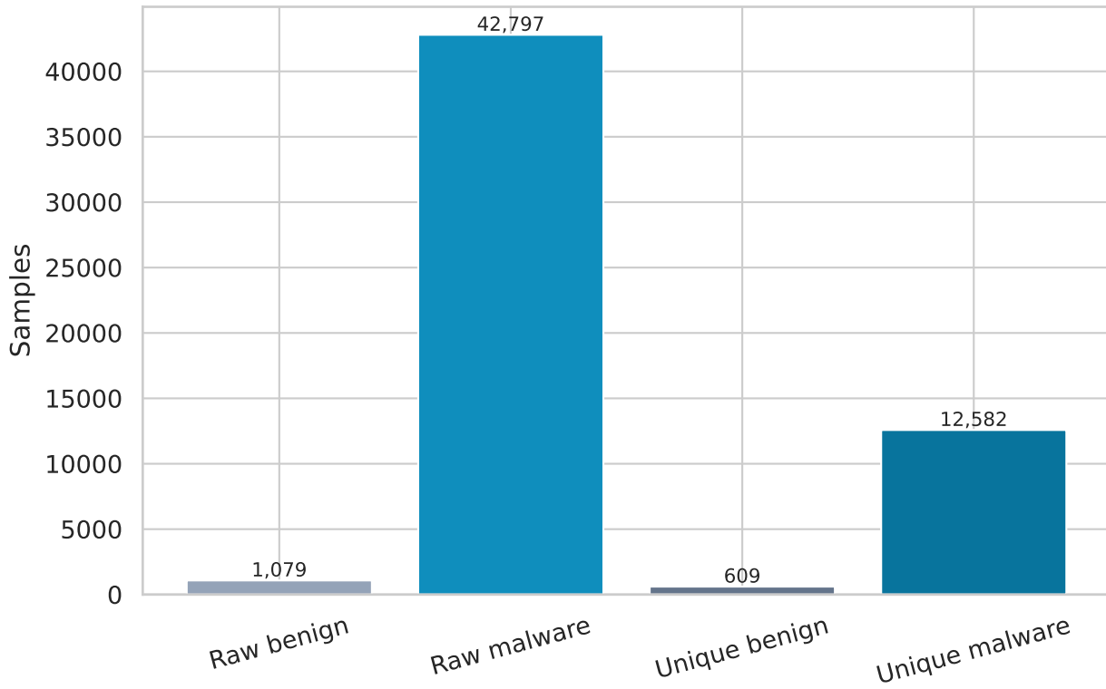
Dataset composition before and after sequence deduplication
