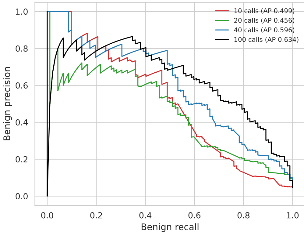
Benign-class precision-recall
