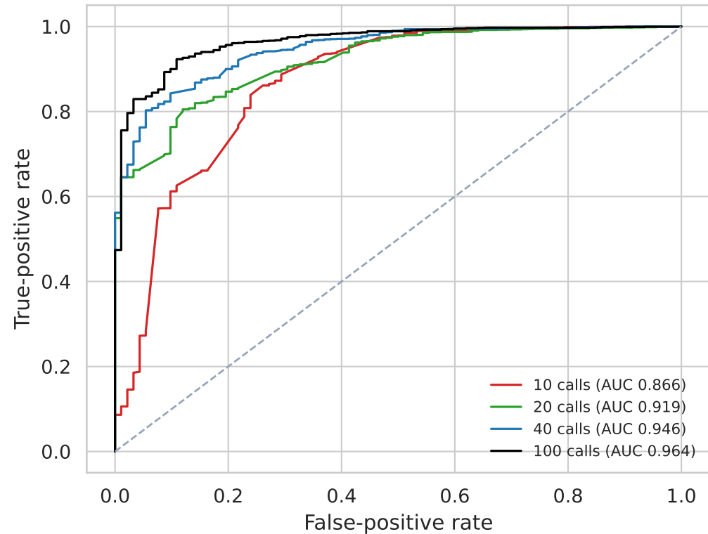
ROC curves
