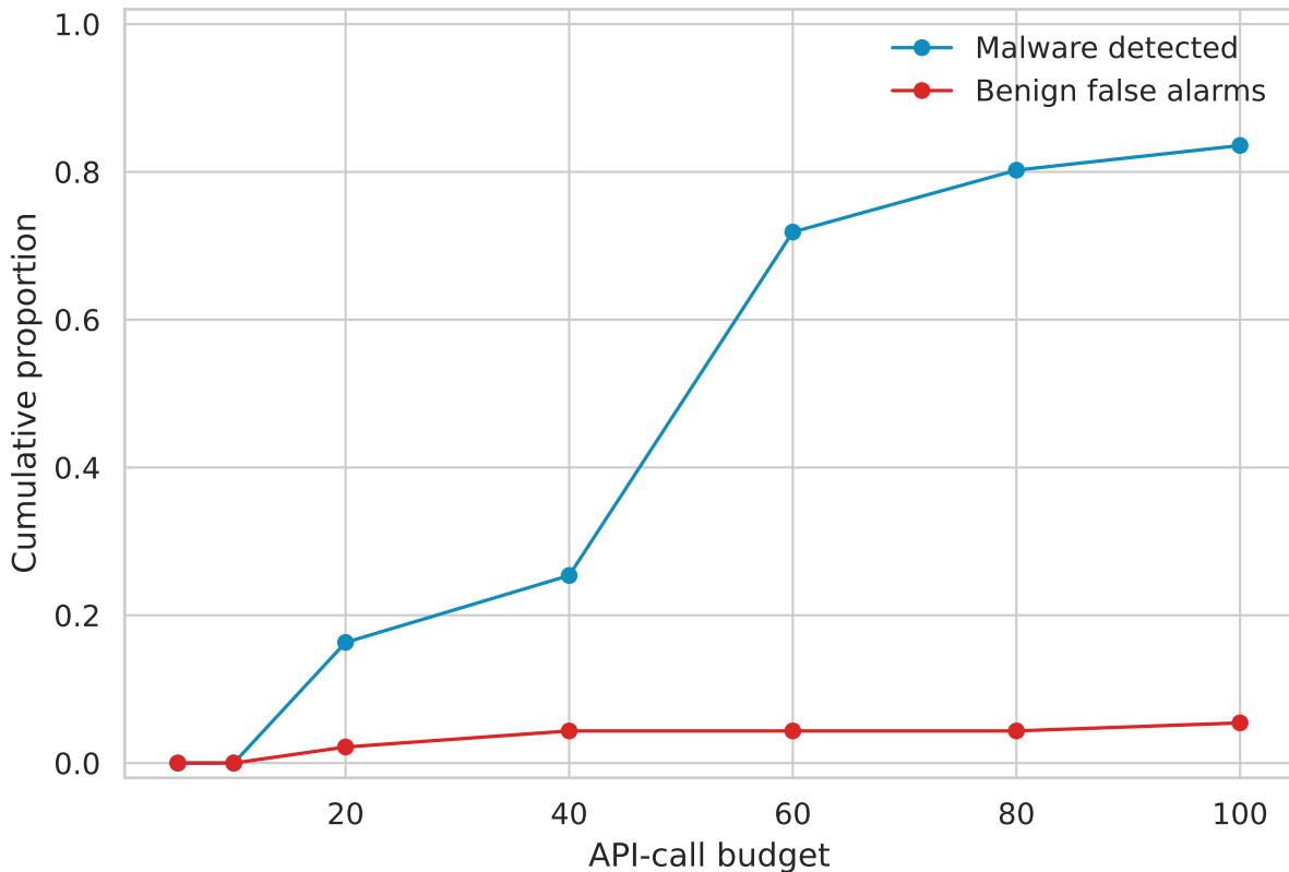
Sequential early-detection policy
