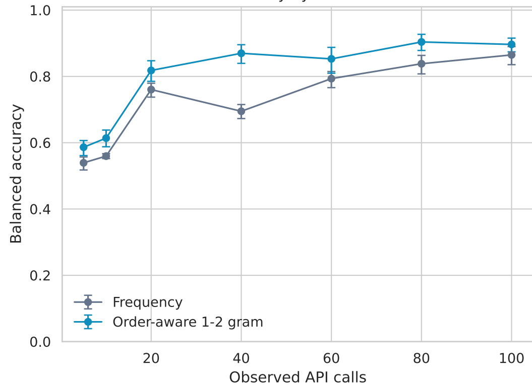
Balanced accuracy by observed API calls
