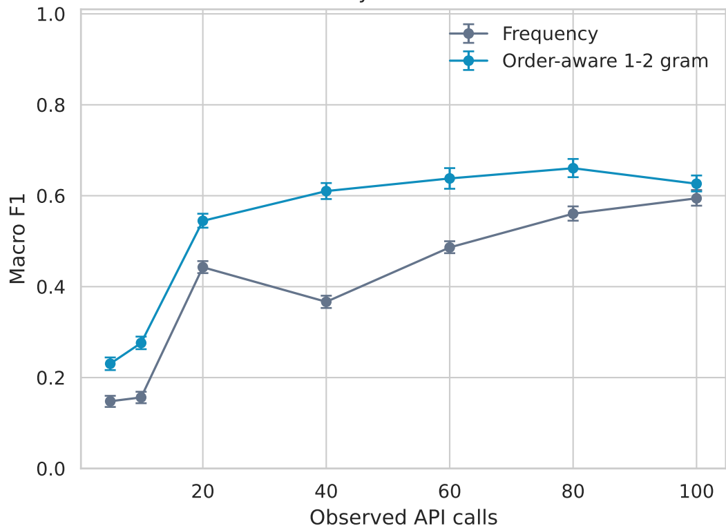
Macro F1 by observed API calls
