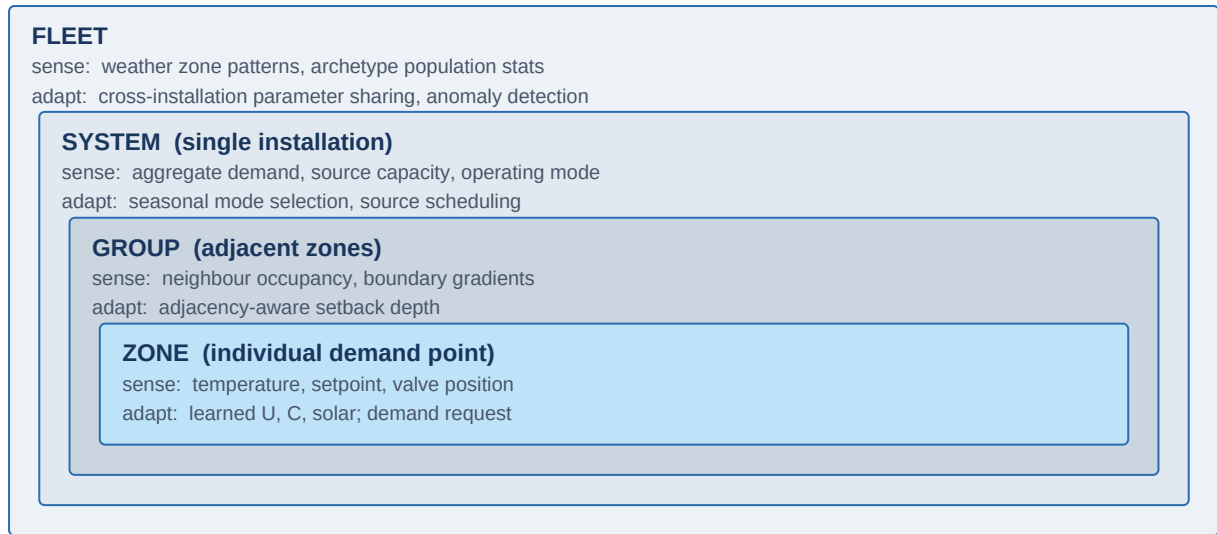
Figure 1: Fractal Self-Similarity Across Scales
