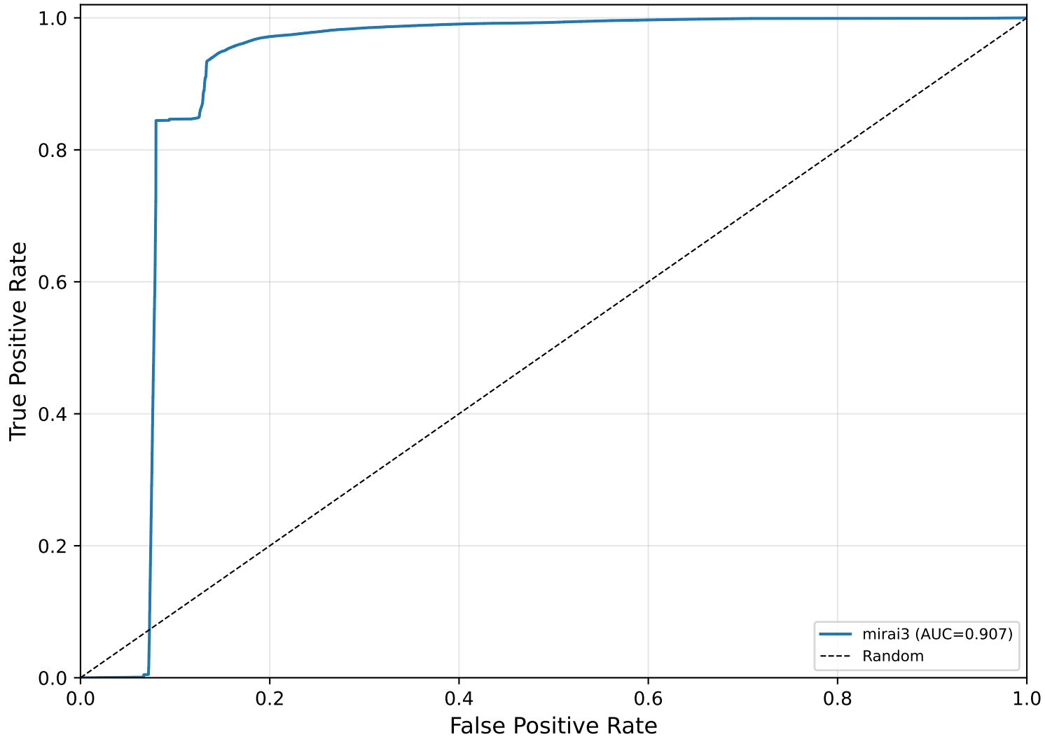
Kitsune-Mirai — ROC Curves
