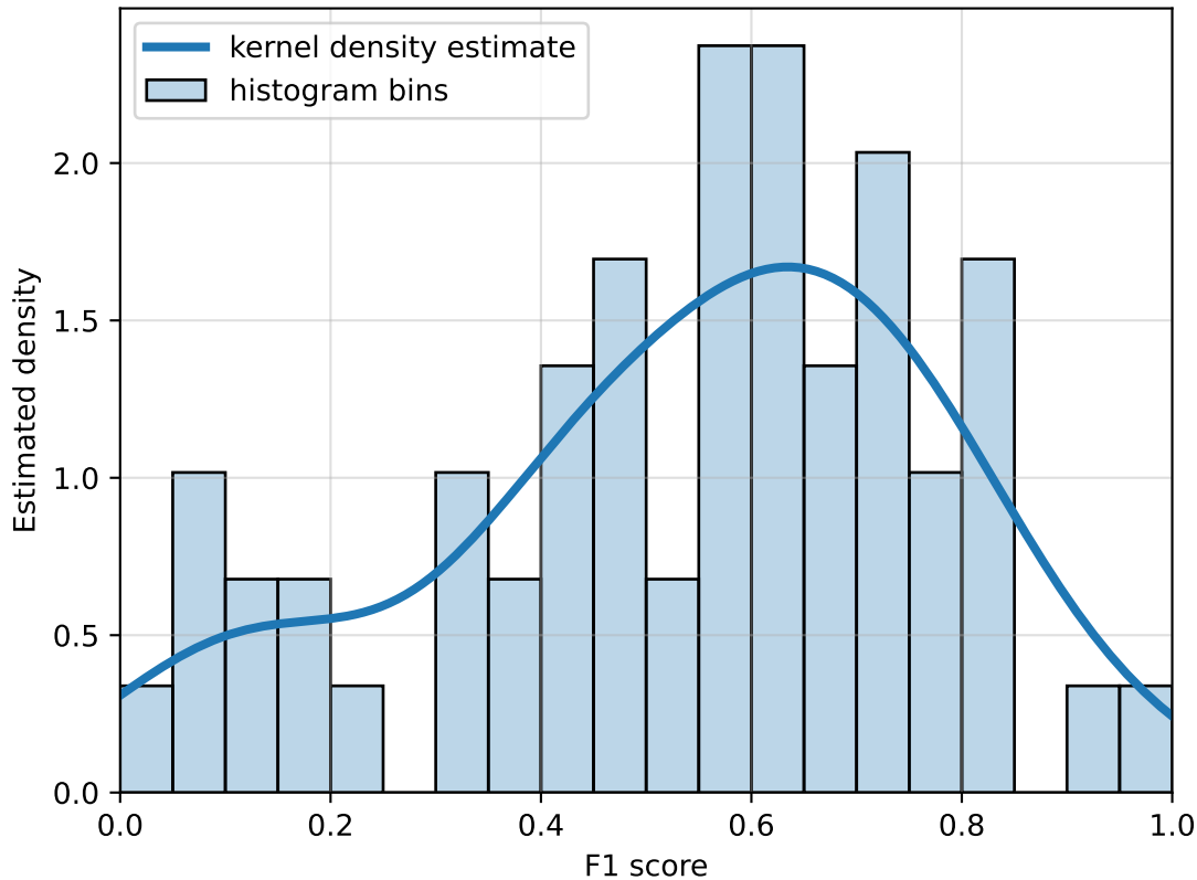
Estimated density of distribution of F1 scores per recording in testset
