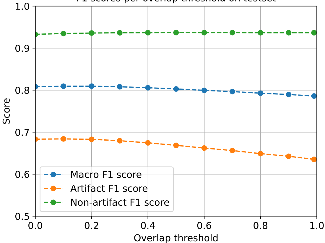
F1 scores per overlap threshold on testset
