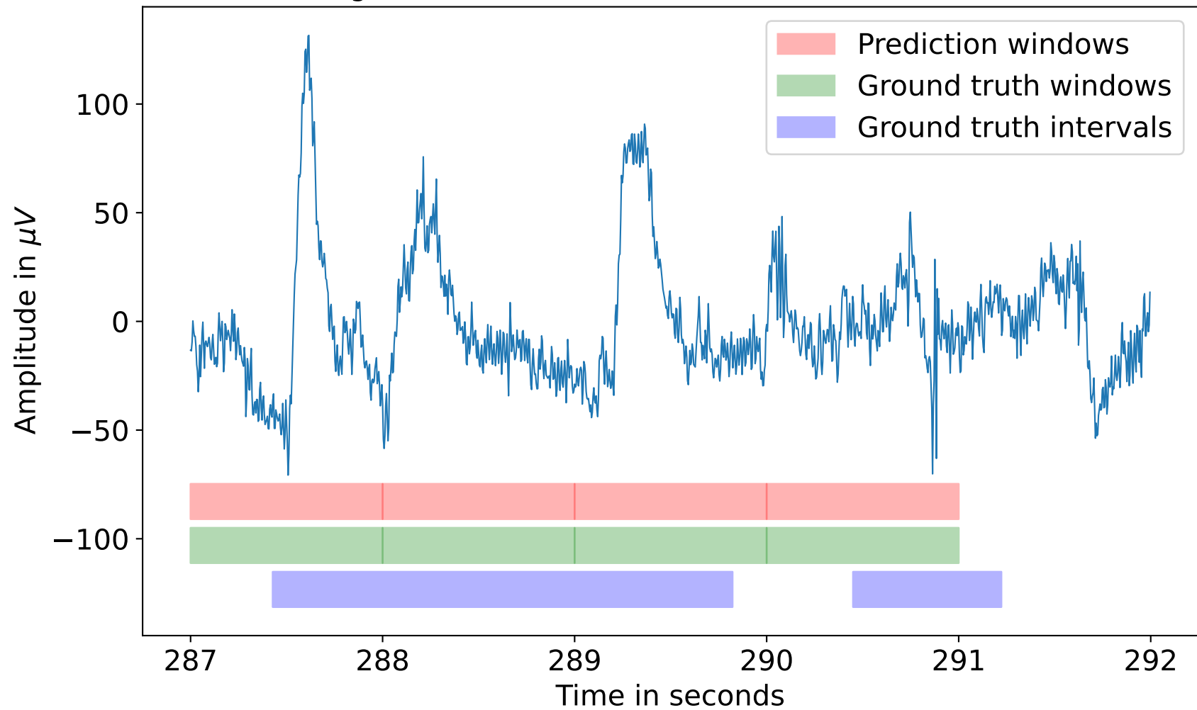
Predictions and ground truth of channel F7-T3 between seconds 287 and 292
