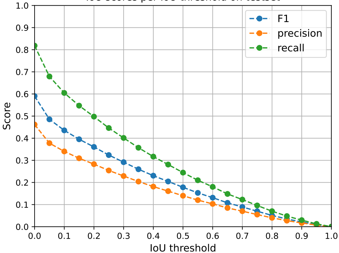
IoU scores per IoU threshold on testset
