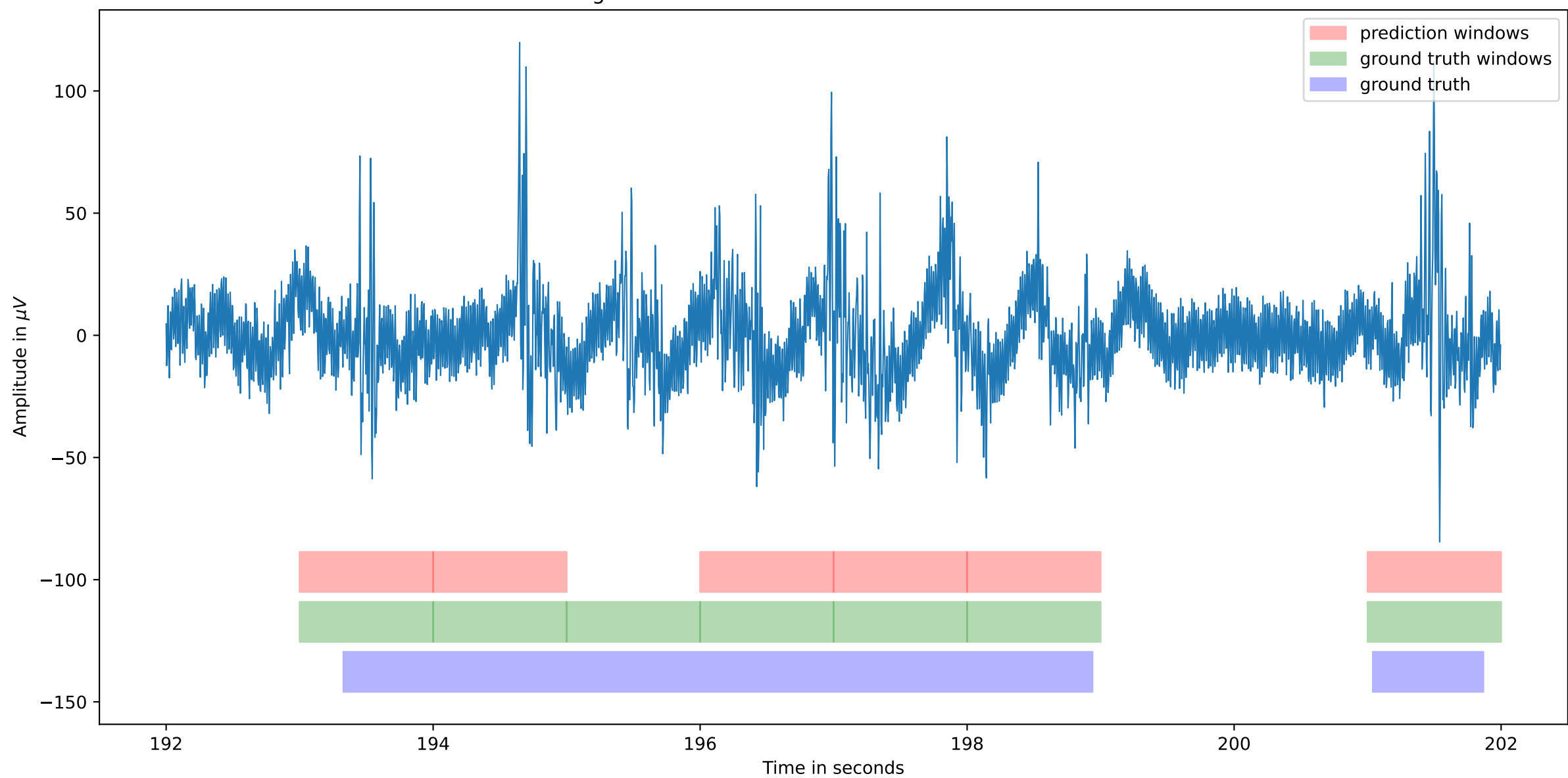
Predictions and ground truth of channel C3-CZ between seconds 192 and 202
