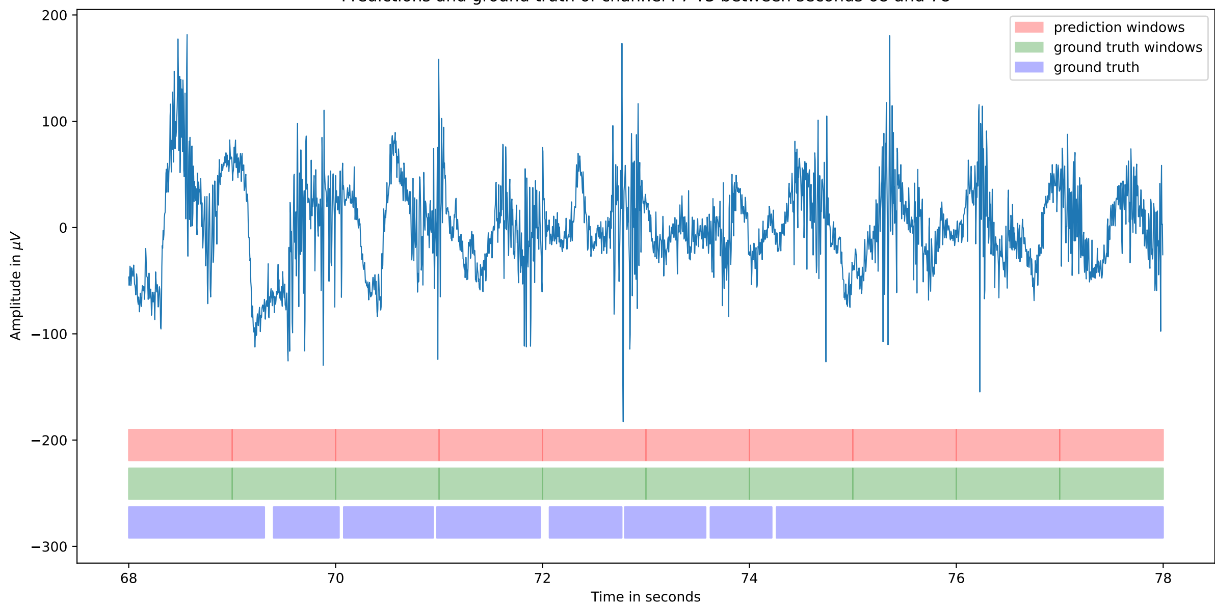
Predictions and ground truth of channel F7-T3 between seconds 68 and 78
