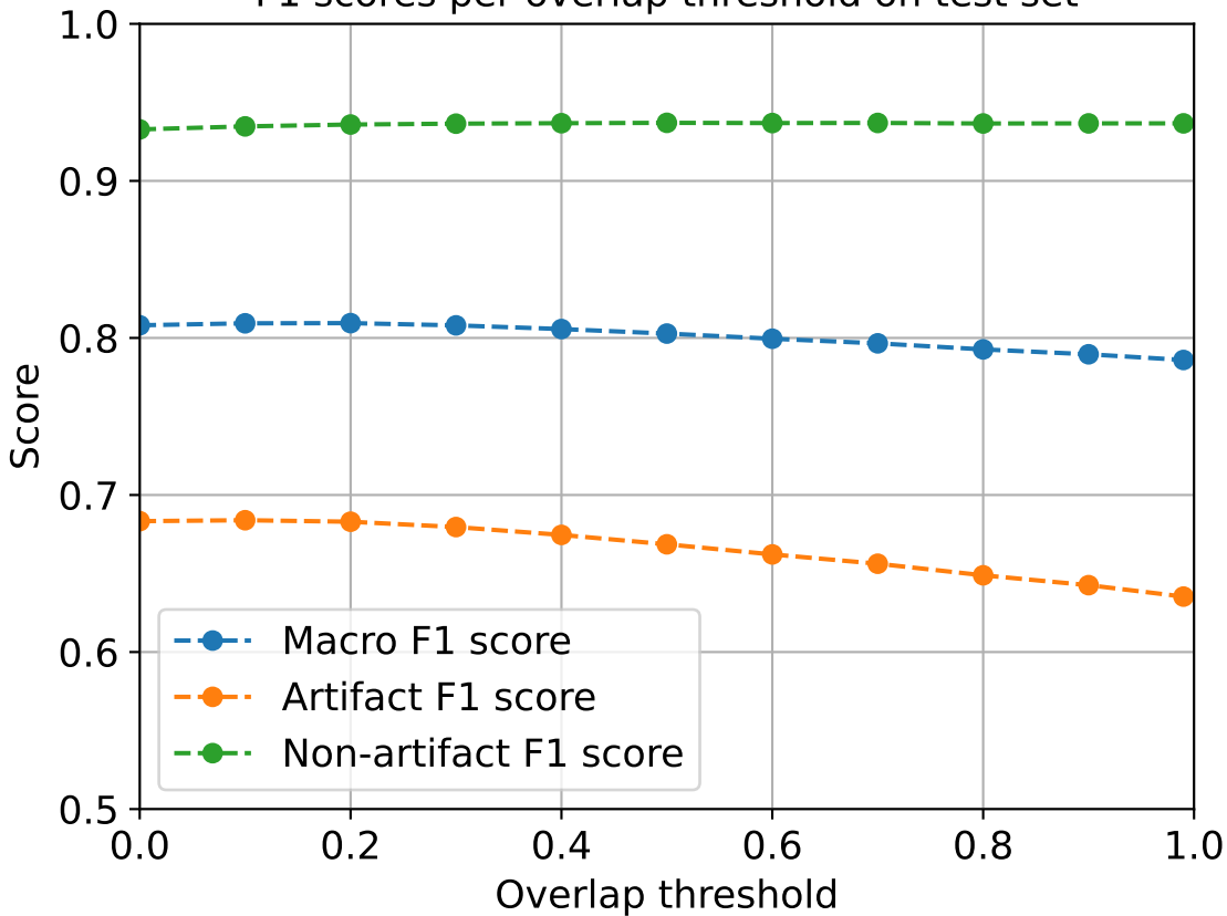
F1 scores per overlap threshold on test set
