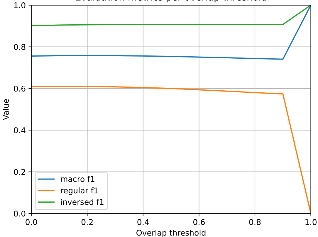
Evaluation metrics per overlap threshold
