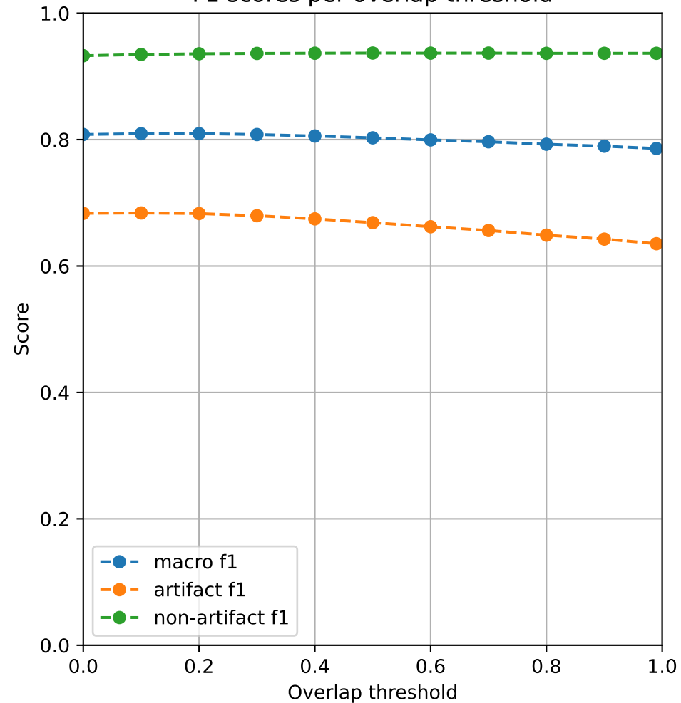
F1 scores per overlap threshold
