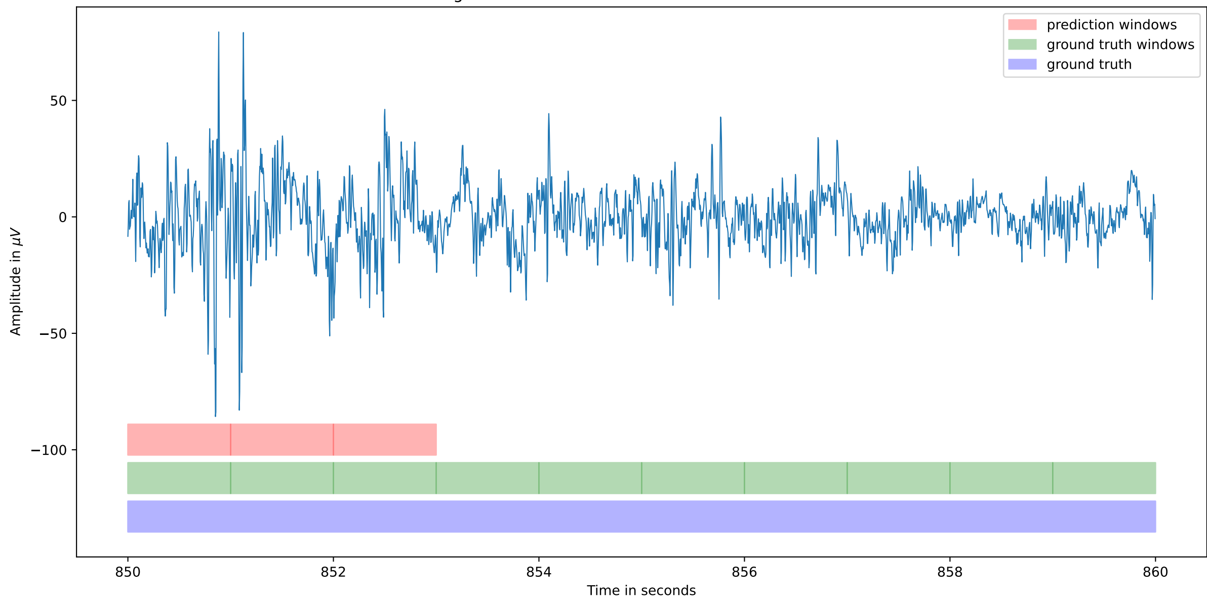
Predictions and ground truth of channel FP1-F7 between seconds 850 and 860
