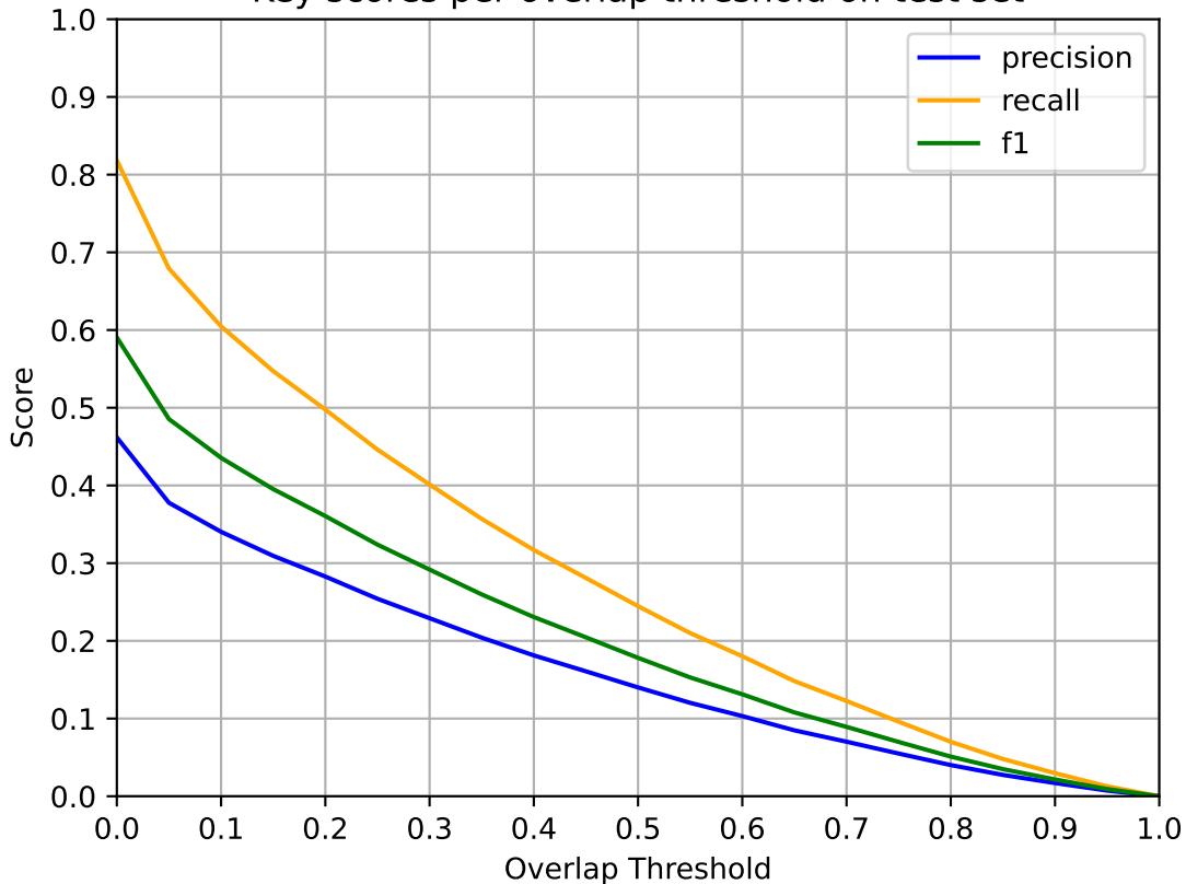
Key scores per overlap threshold on test set
