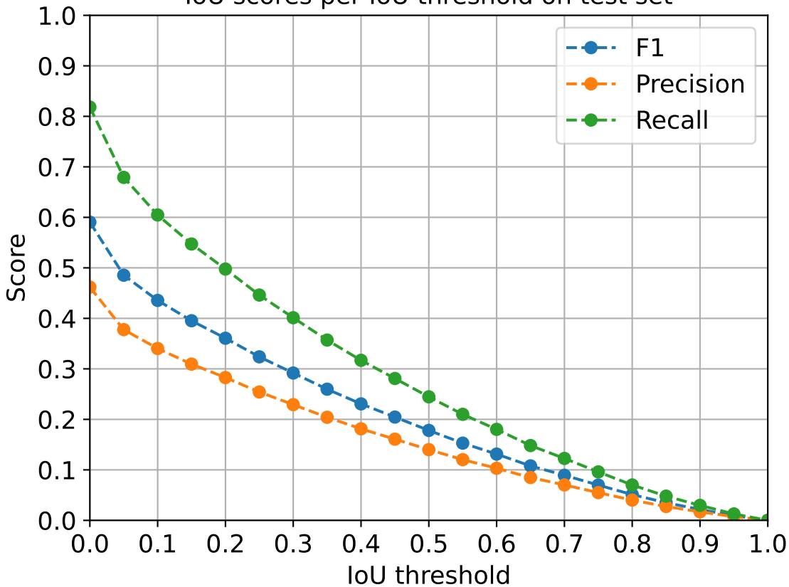
IoU scores per IoU threshold on test set
