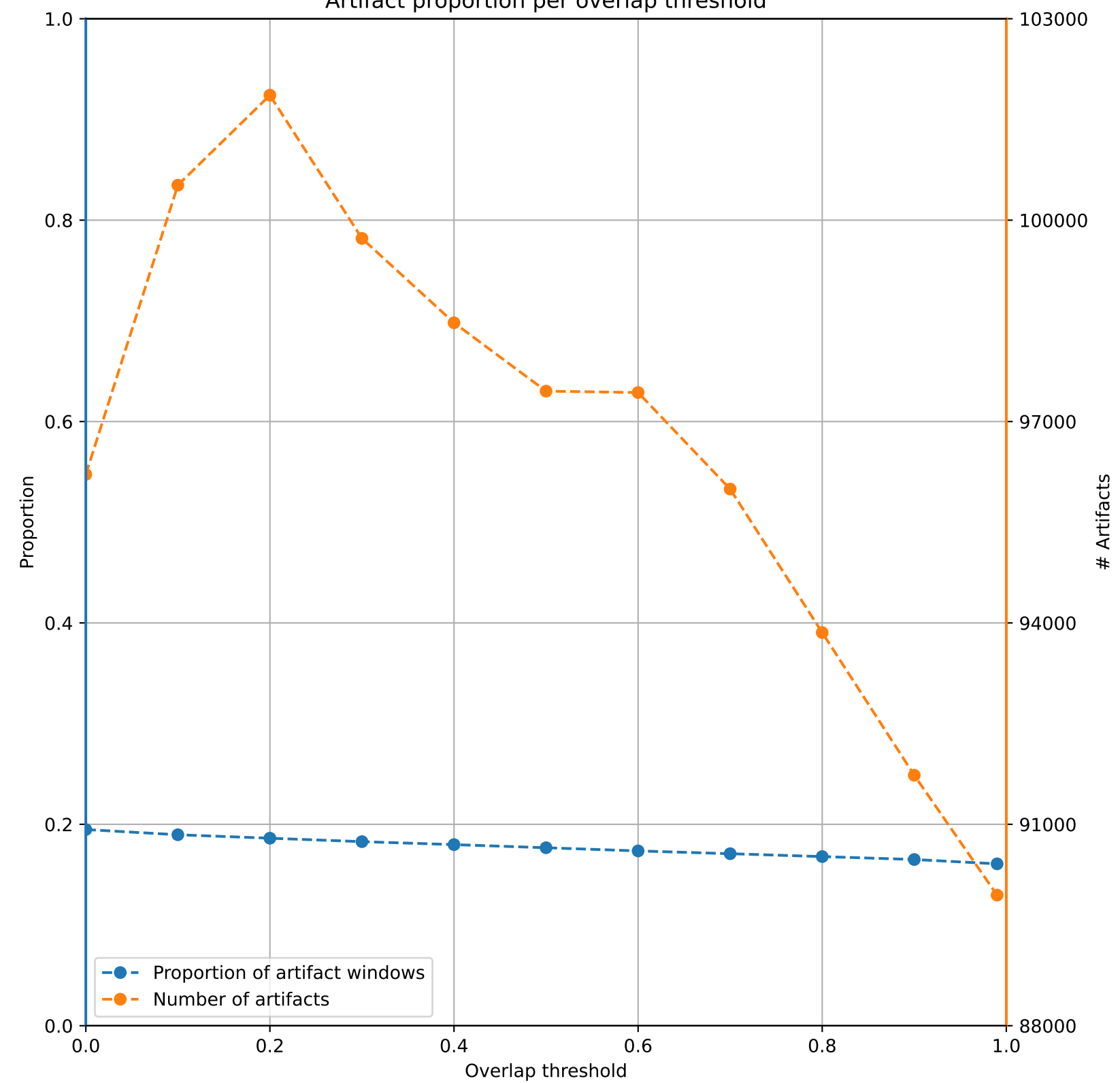
Artifact proportion per overlap threshold
