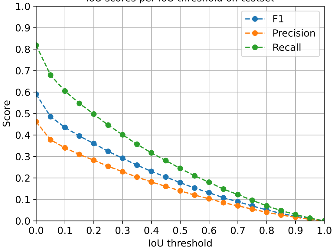
IoU scores per IoU threshold on testset
