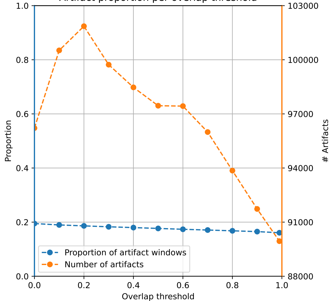
Artifact proportion per overlap threshold
