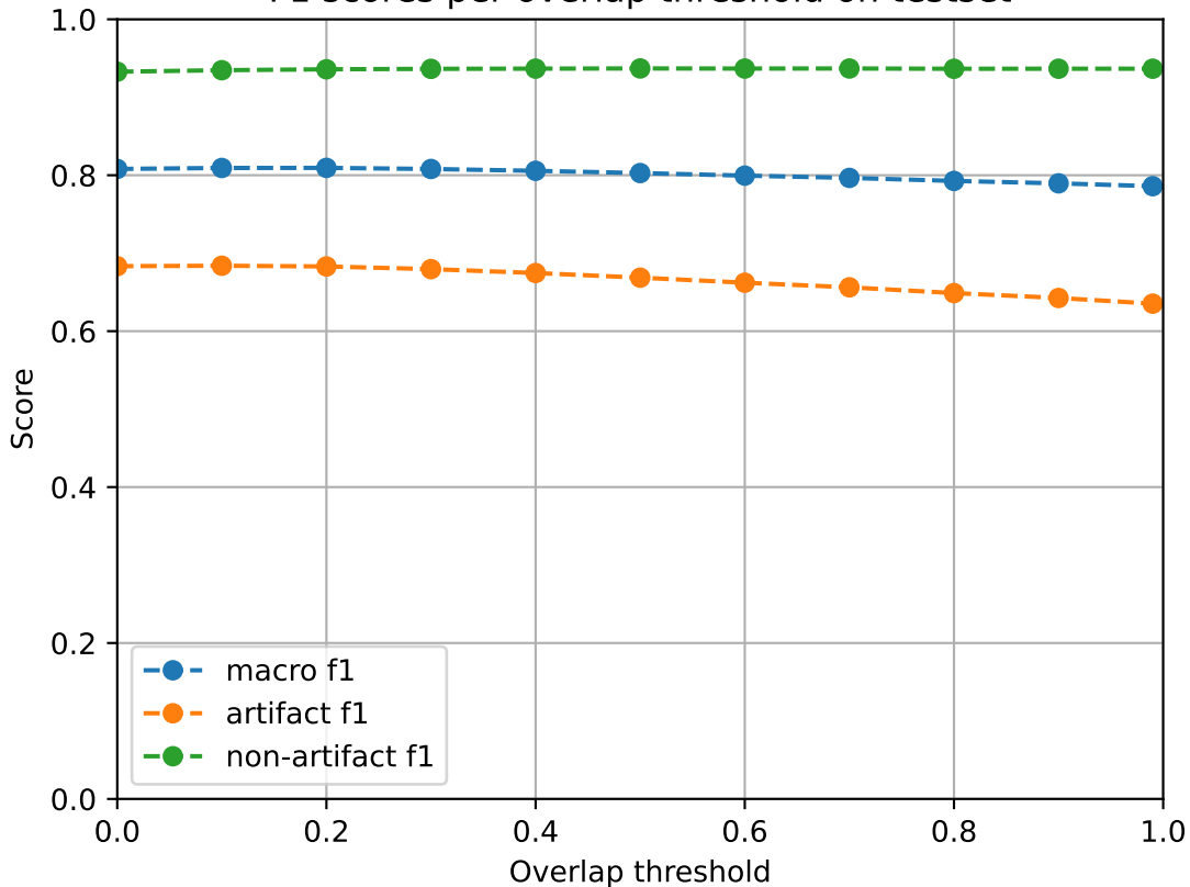
F1 scores per overlap threshold on testset
