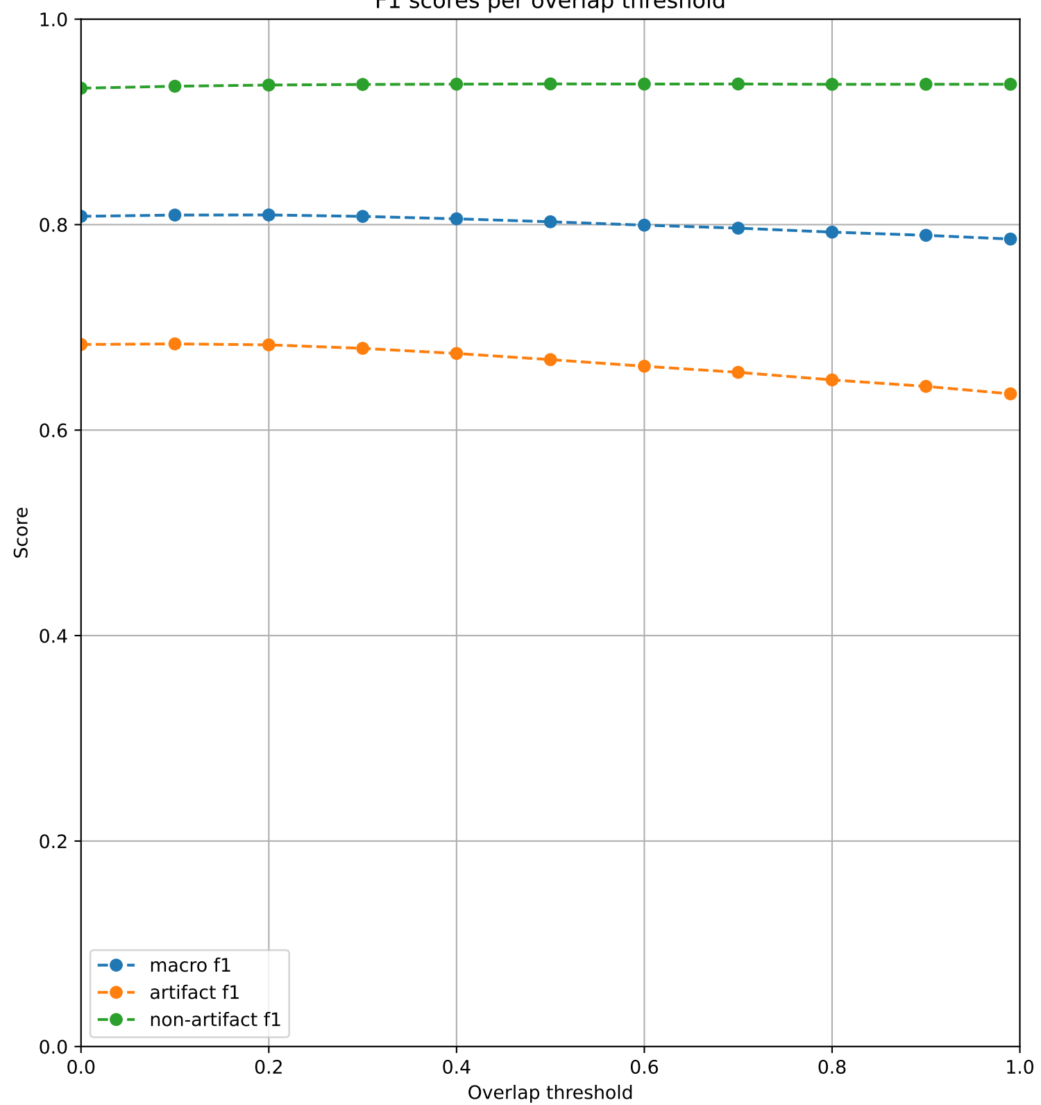
F1 scores per overlap threshold
