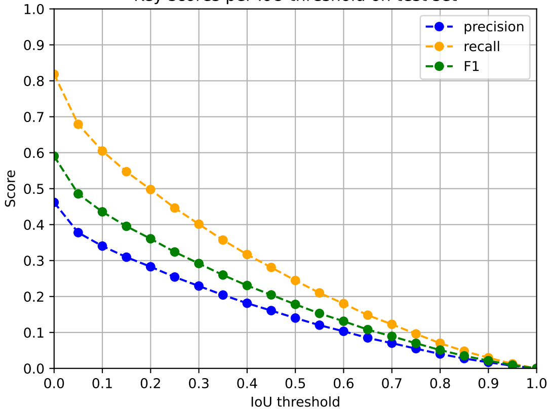
Key scores per IoU threshold on test set
