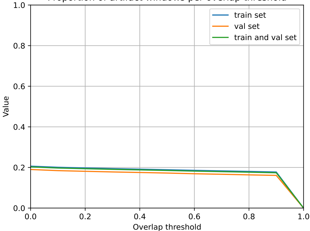
Proportion of artifact windows per overlap threshold
