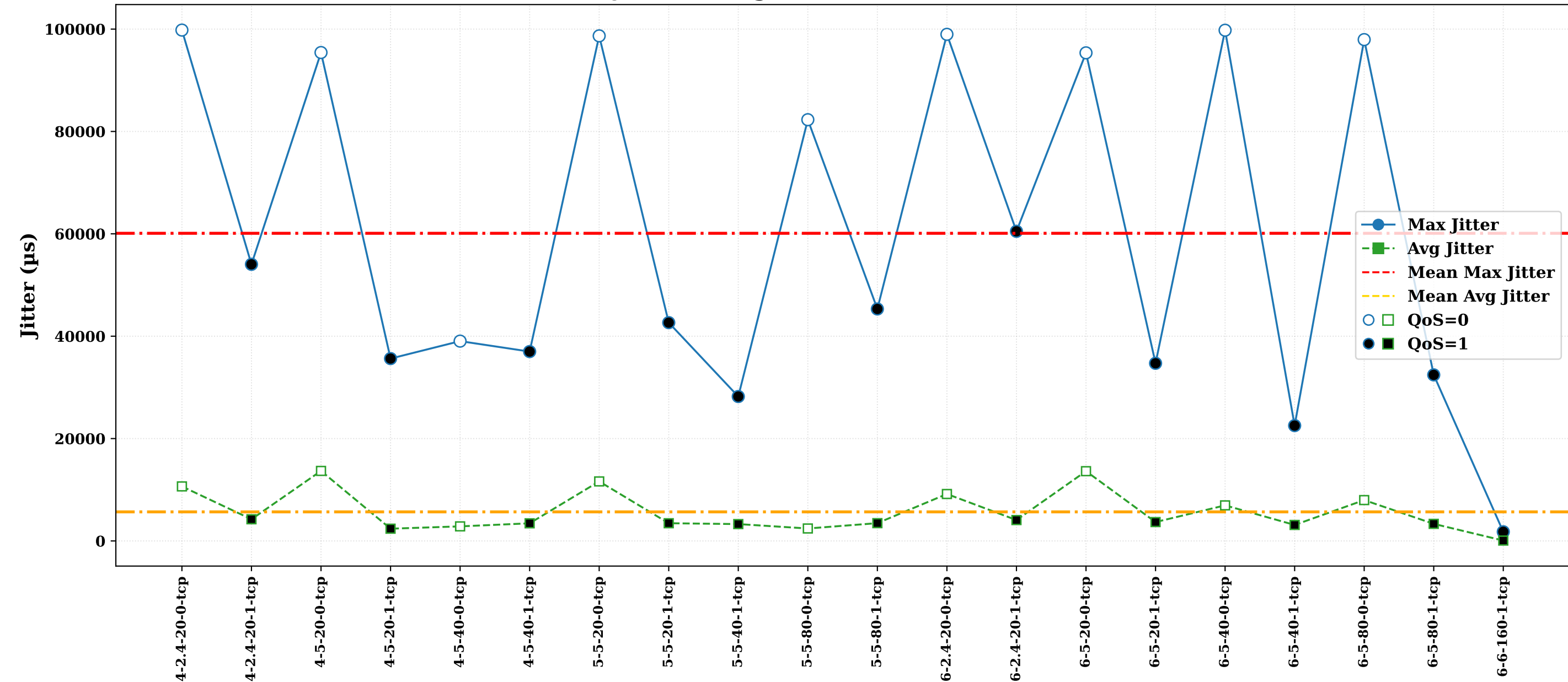
Jitter for high disturbance test (TCP)
