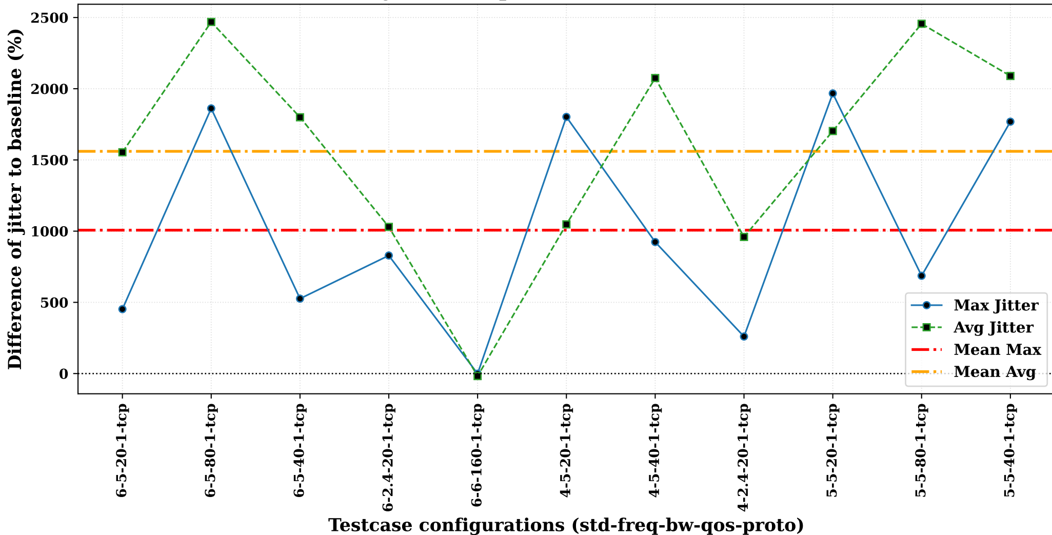
Jitter comparison for TCP cases
