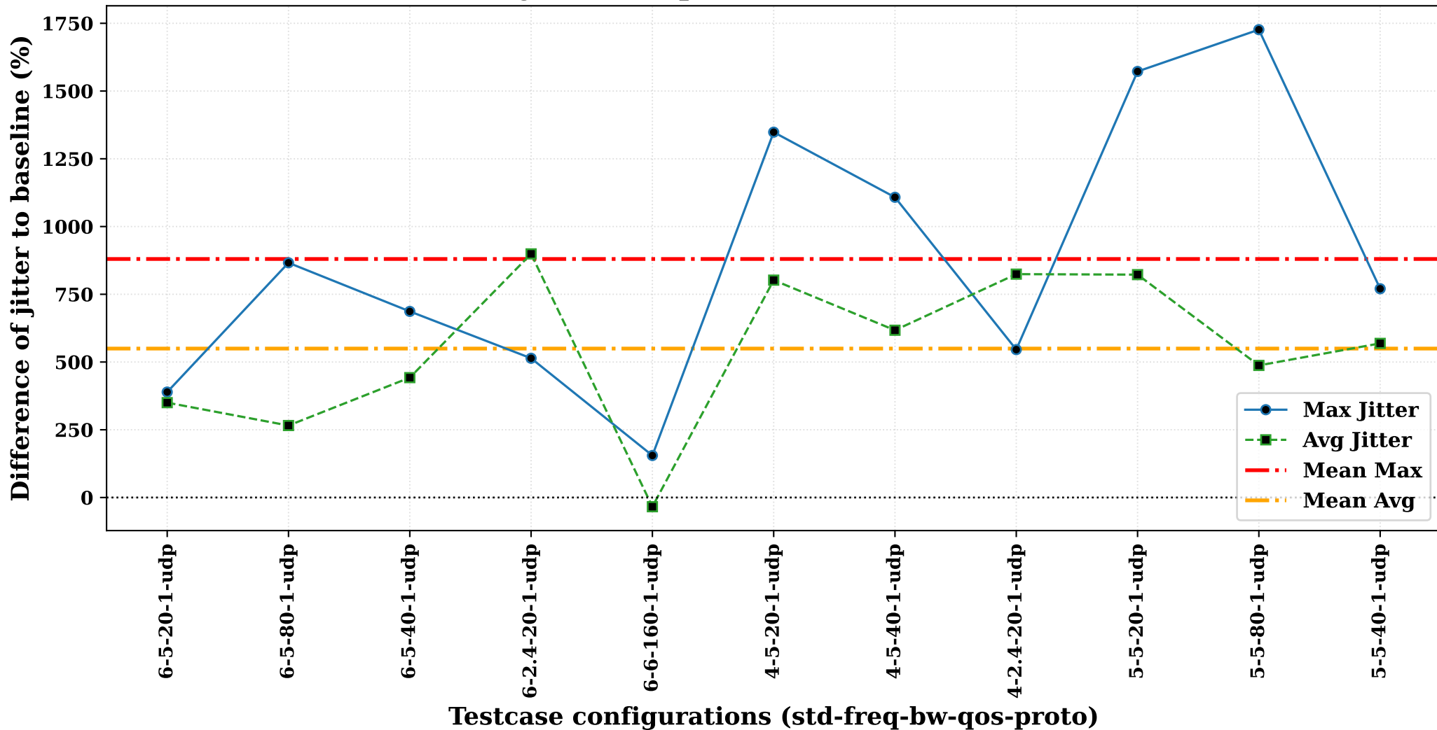
Jitter comparison for UDP cases
