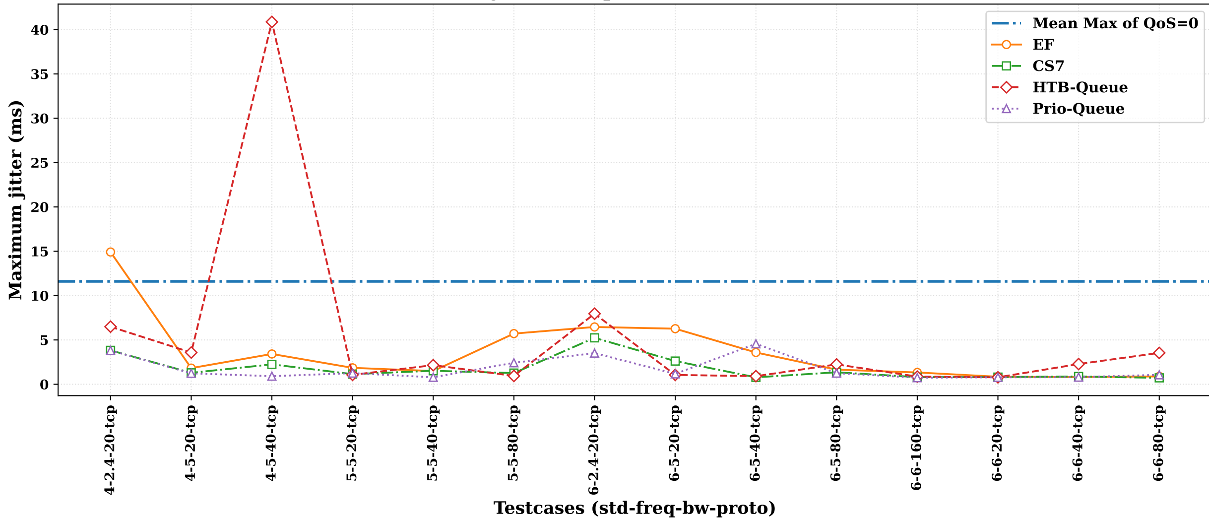
Jitter comparison for TCP
