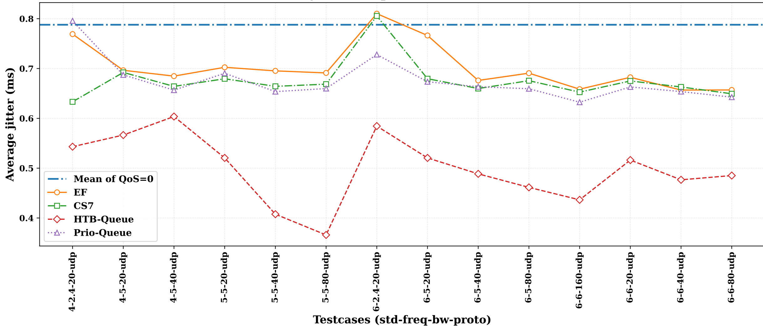
Jitter comparison for UDP
