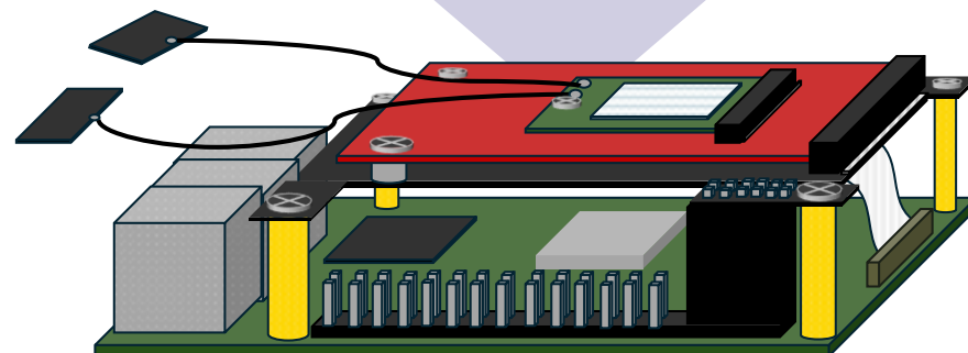
Client
