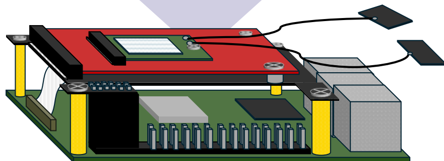
Server
