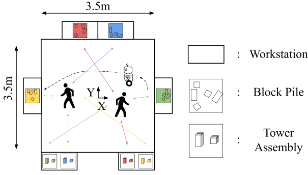
Figure 2: Experimental setup. Each participant is responsible for assembling towers from two different colored (green and red or yellow and blue) piles of blocks, while the robot traverses the workspace between stations. The color ordering is fixed so the green and yellow towers are completed before the red and blue.
