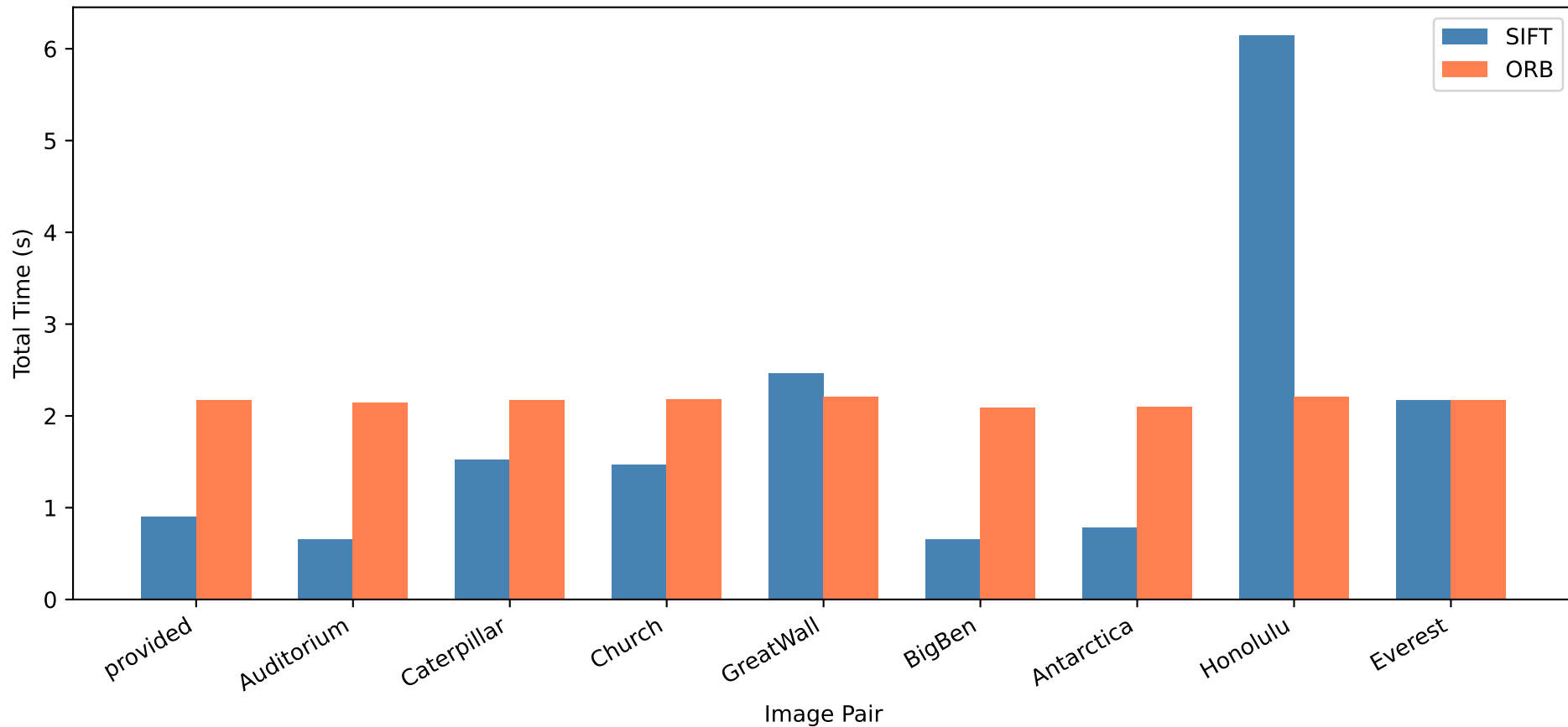
SIFT vs ORB: Detection + Matching Speed
