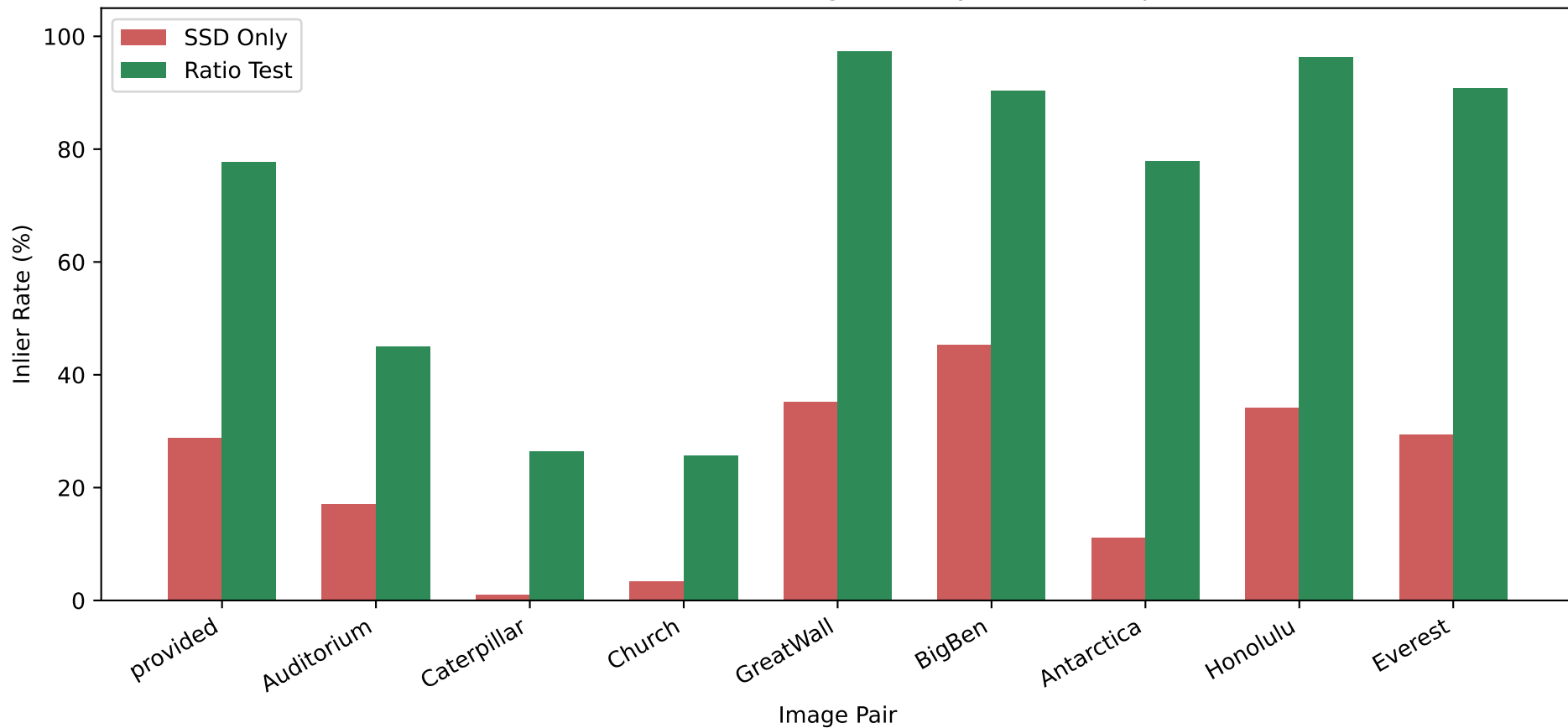
SSD vs Ratio Test: Matching Accuracy (SIFT Descriptor)
