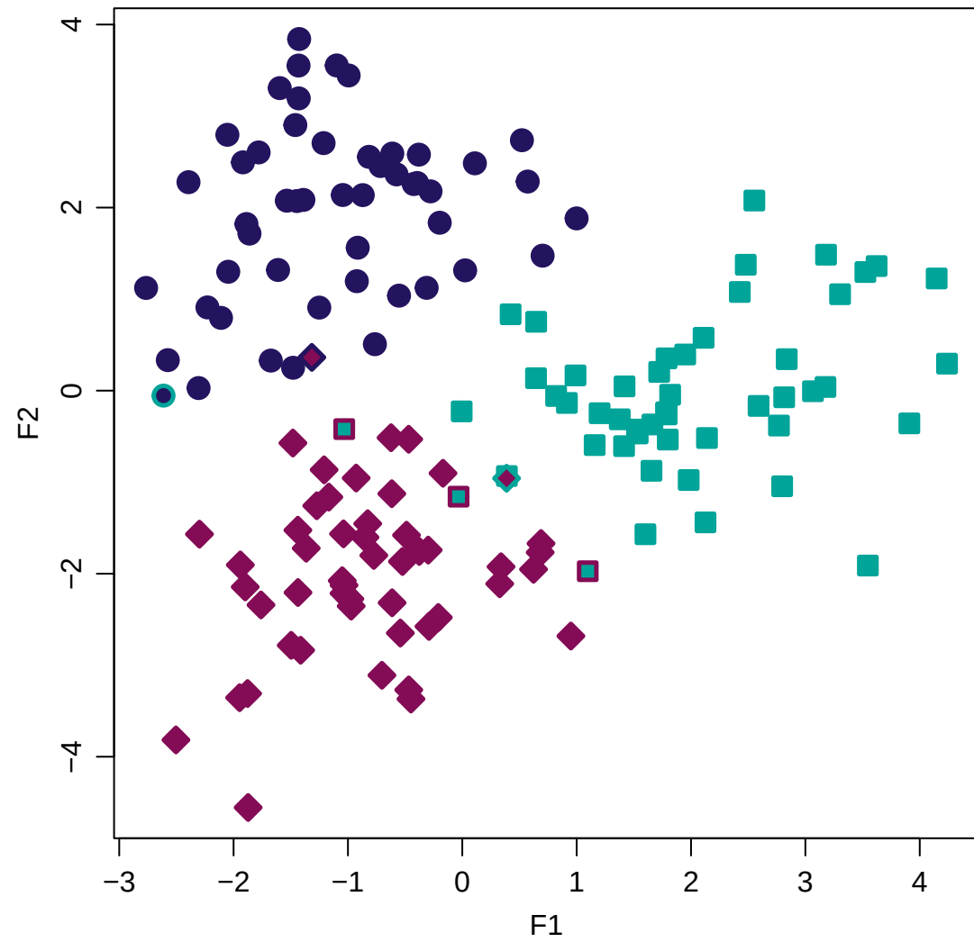
Predicted Clusters via Stability Clustering
