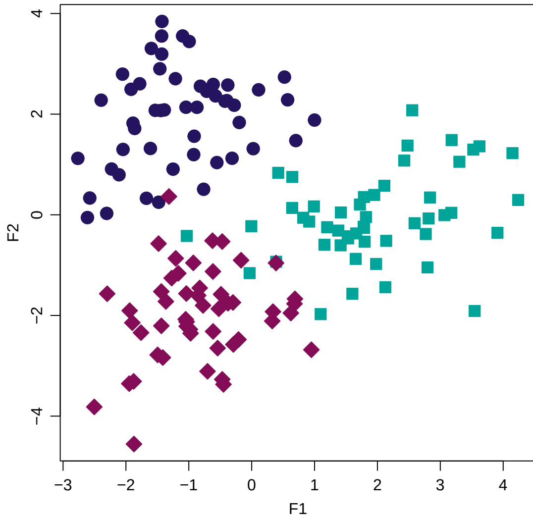
Orig. Simulated 3 Cluster Data
