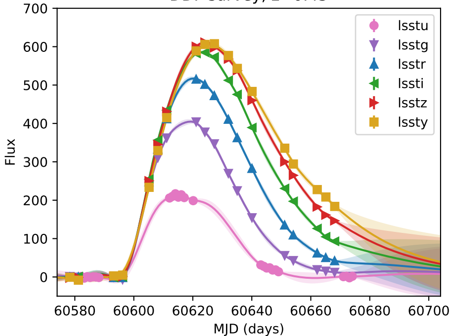
DDF survey, z=0.43
