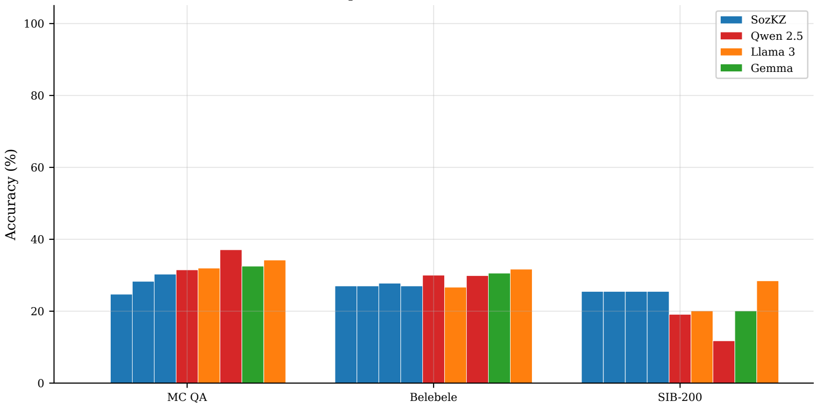
Model Comparison Across Kazakh NLP Tasks
