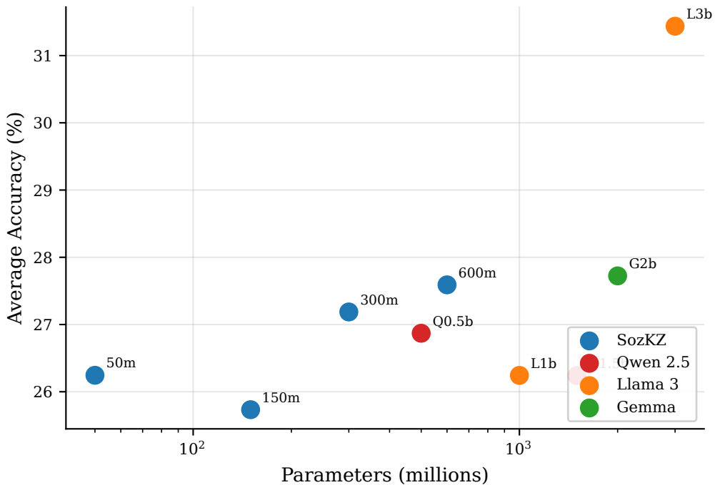
Performance vs Model Size
