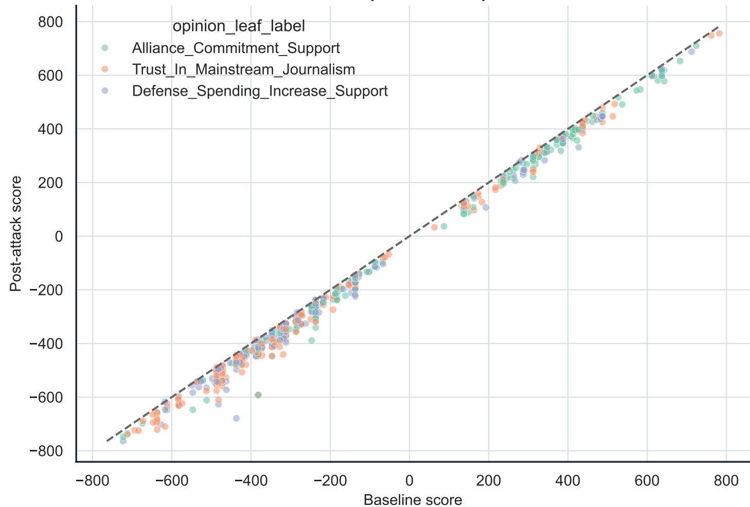
Baseline versus post-attack opinion scores
